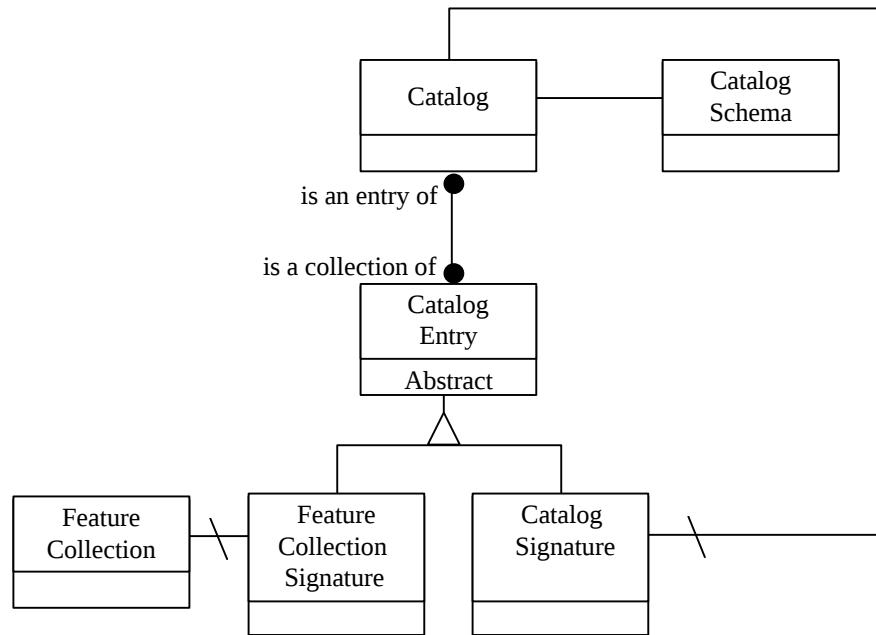
Figure 2-4. Object Types near the Catalog
