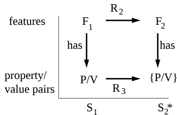
Figure 2-1. The canonical map.
