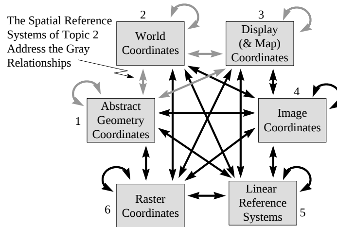
Figure 2-2. Example Domains and Ranges for Locational Geometry Functions
