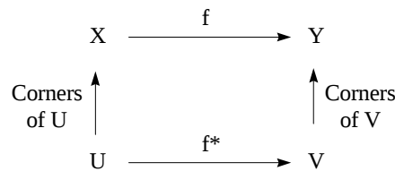
Figure 2-1. The Canonical Mapping
