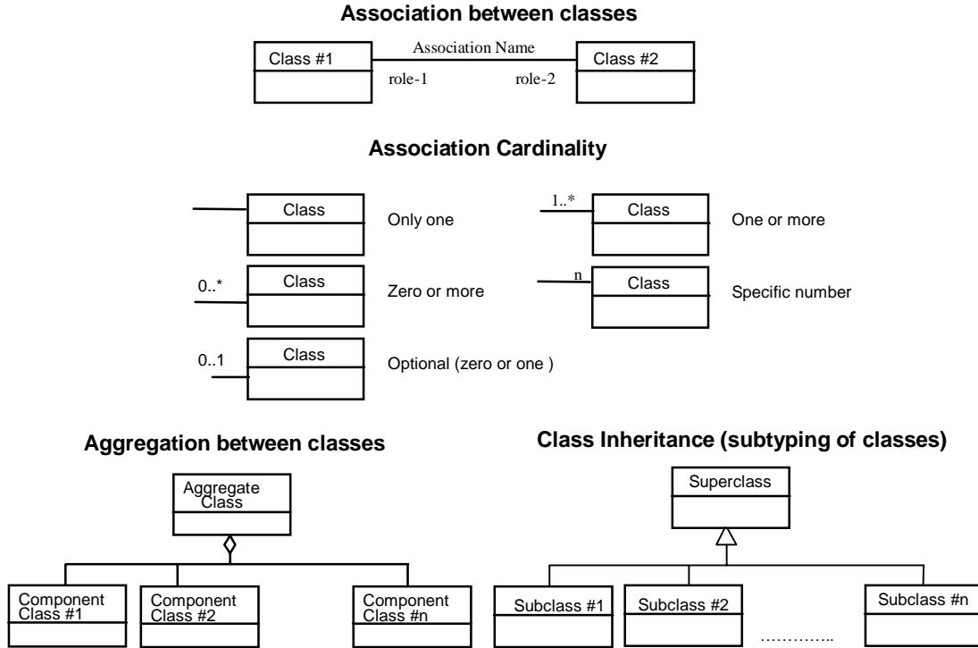
Figure 1 — UML notations
