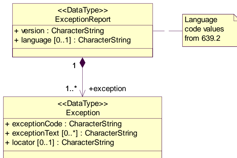
Figure B.6 — OWS Exception Report UML package
