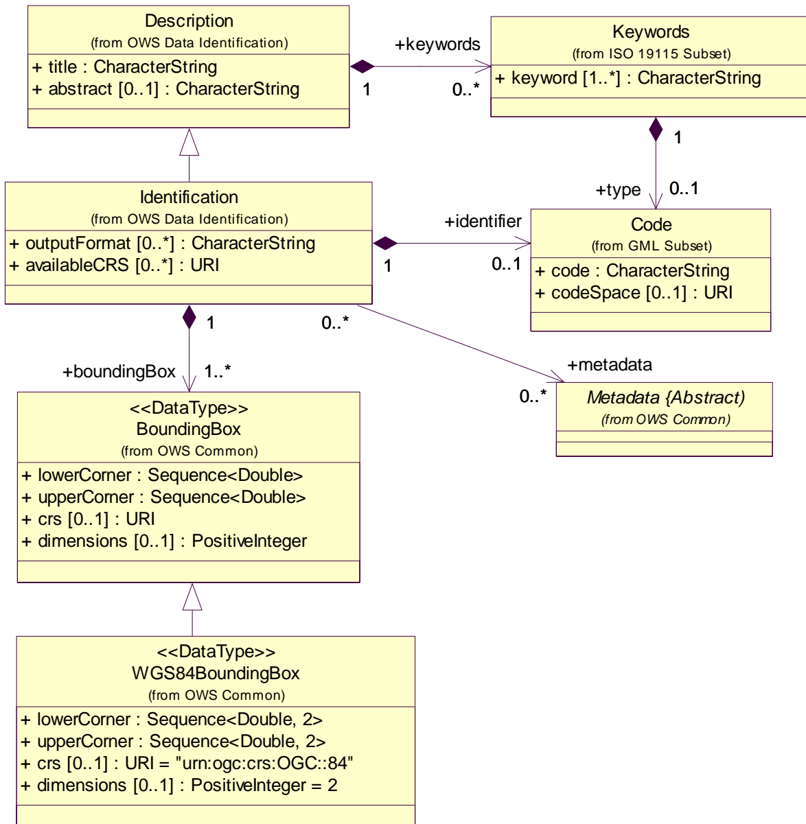
Figure B.7 — OWS Data Identification and Common UML packages
