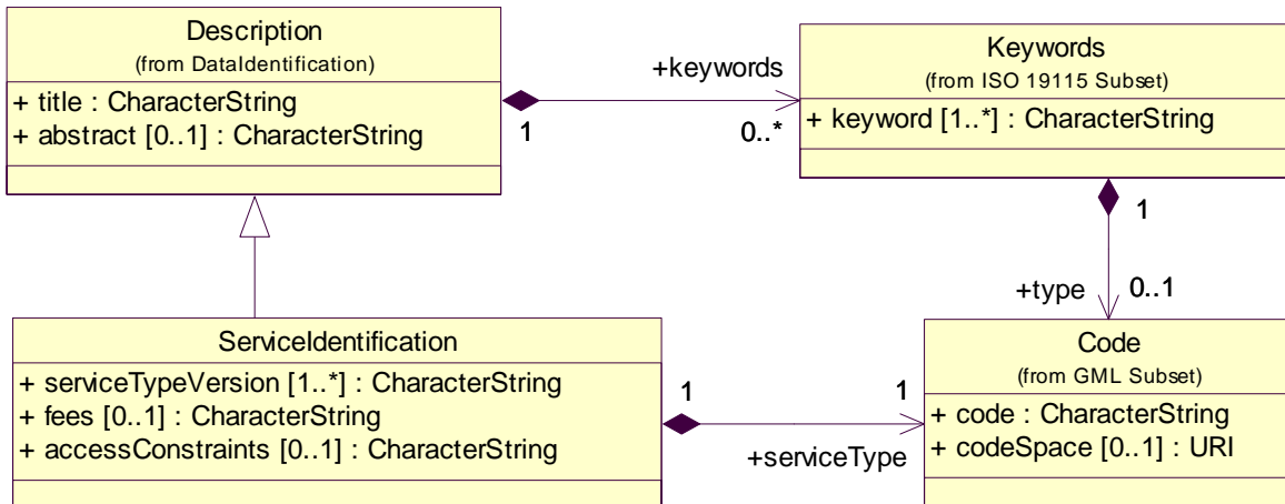
Figure B.5 — OWS Service Identification UML package
