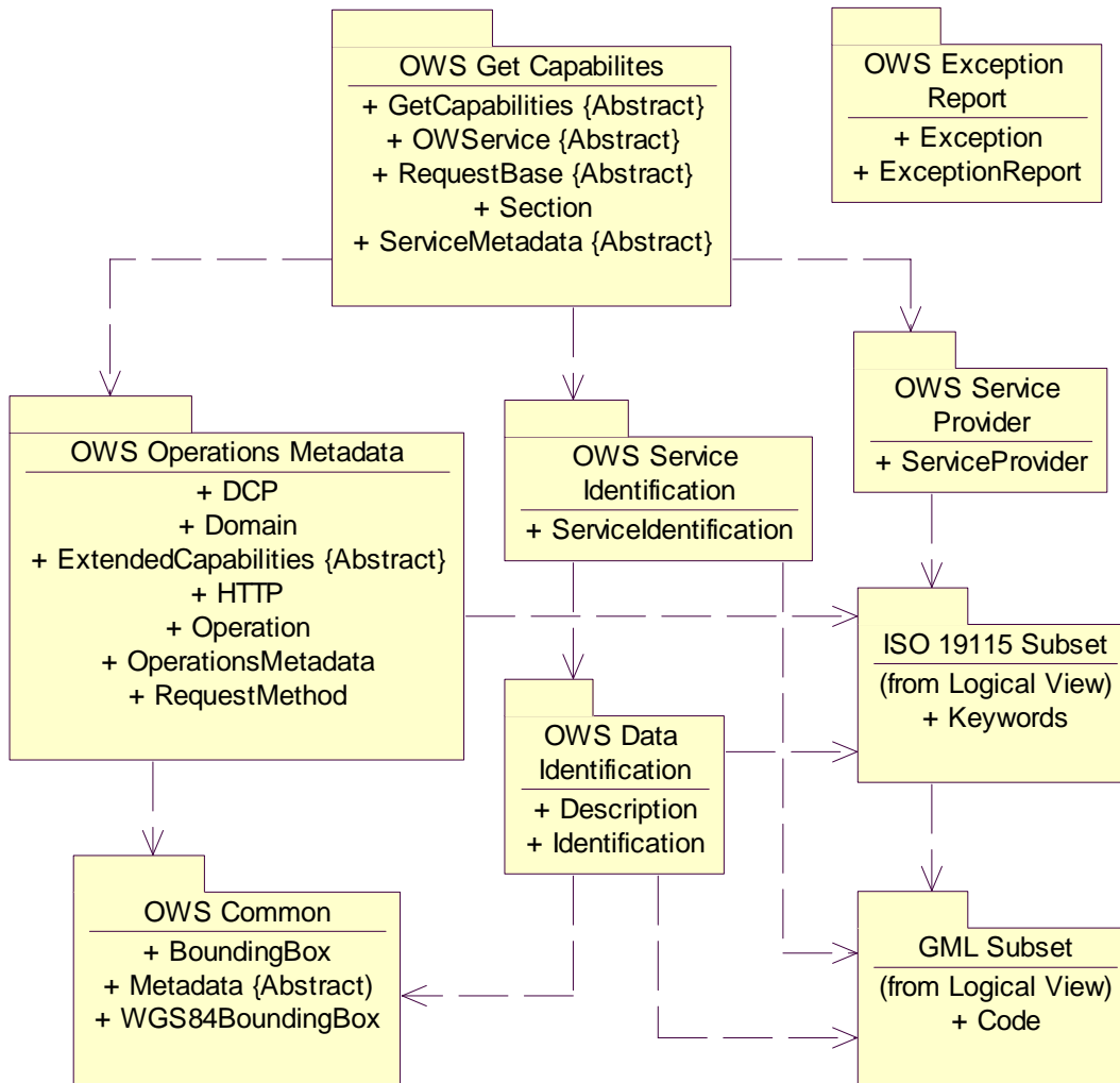
Figure B.1 — OWS Common UML package diagram
