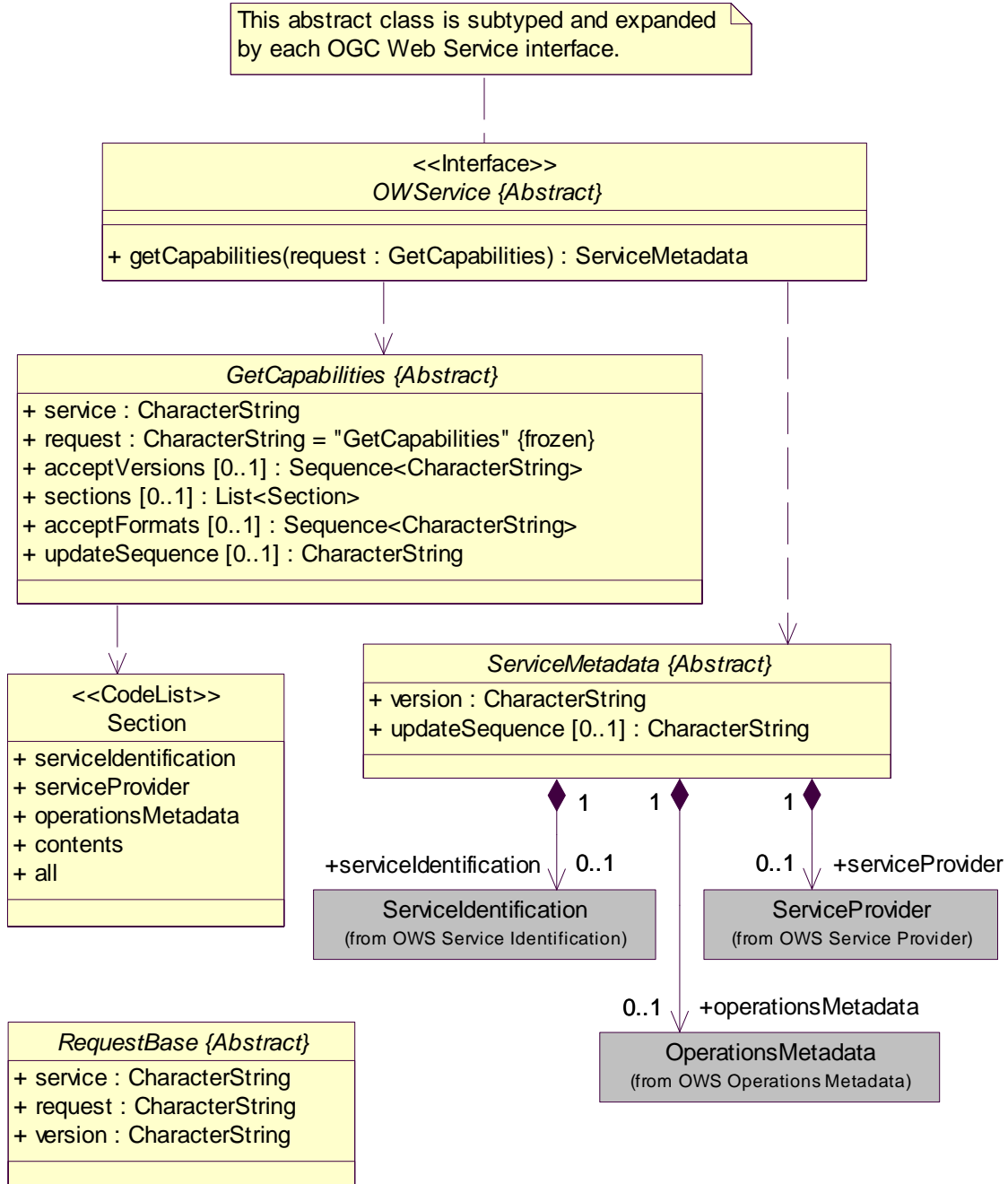
Figure B.2 — OWS Get Capabilities UML package
