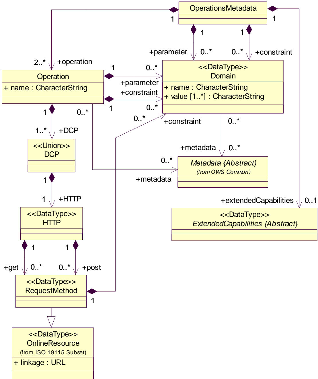
Figure B.4 — OWS Operations Metadata UML package
