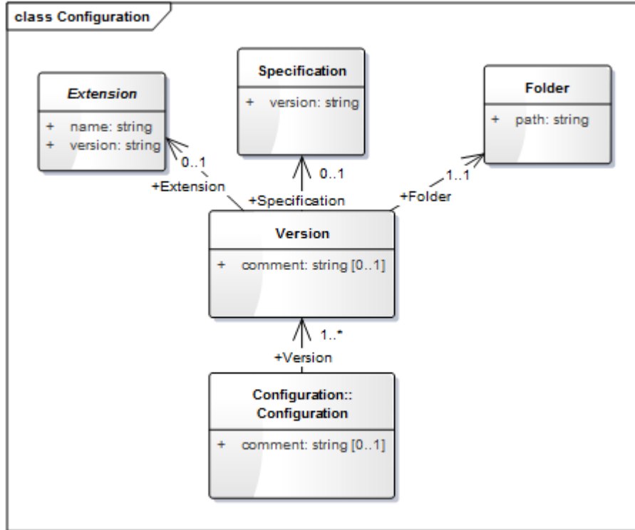
Figure 17: UML diagram of configuration metadata
