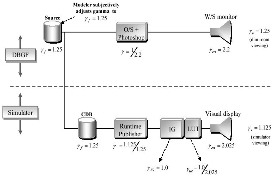
Figure 6-1: Typical Handling of Gamma at DBGF and Simulator
