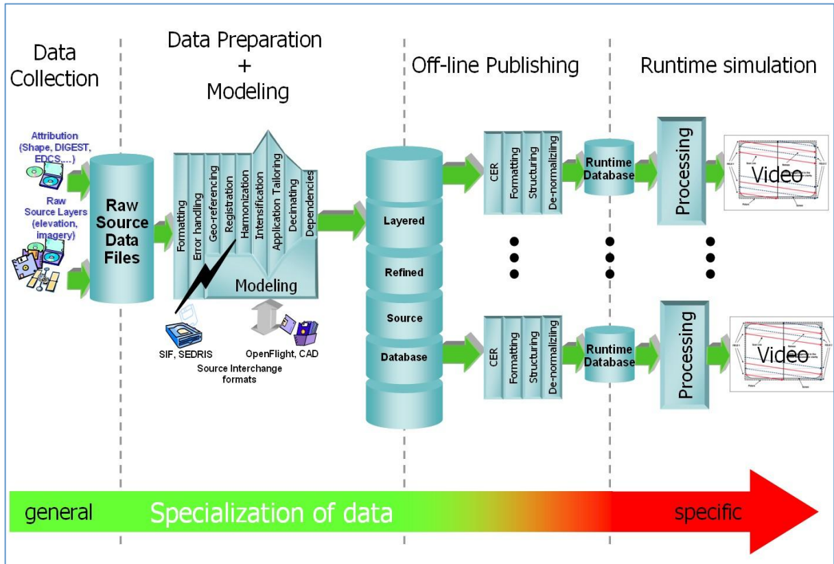
Figure 1- 2: SE Workflow with CDB as an off-line Repository
