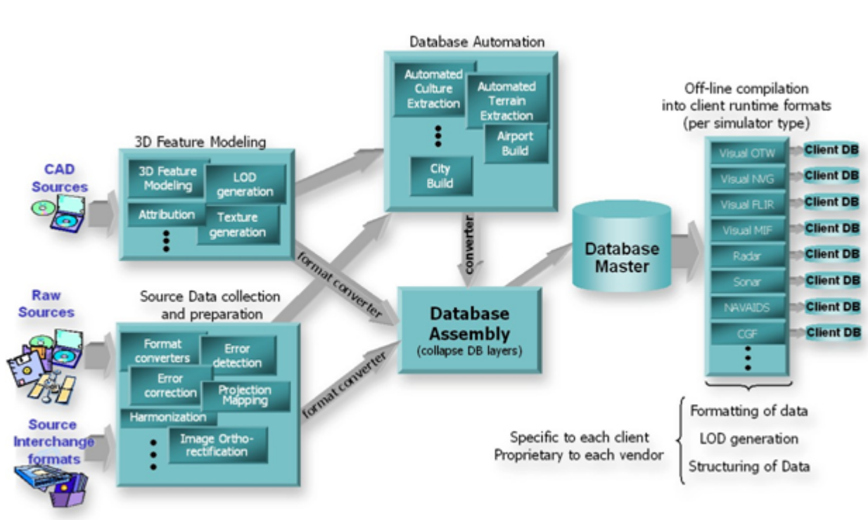
Figure 1- 6: Typical DB Generation - CDB Used as a DB Repository
