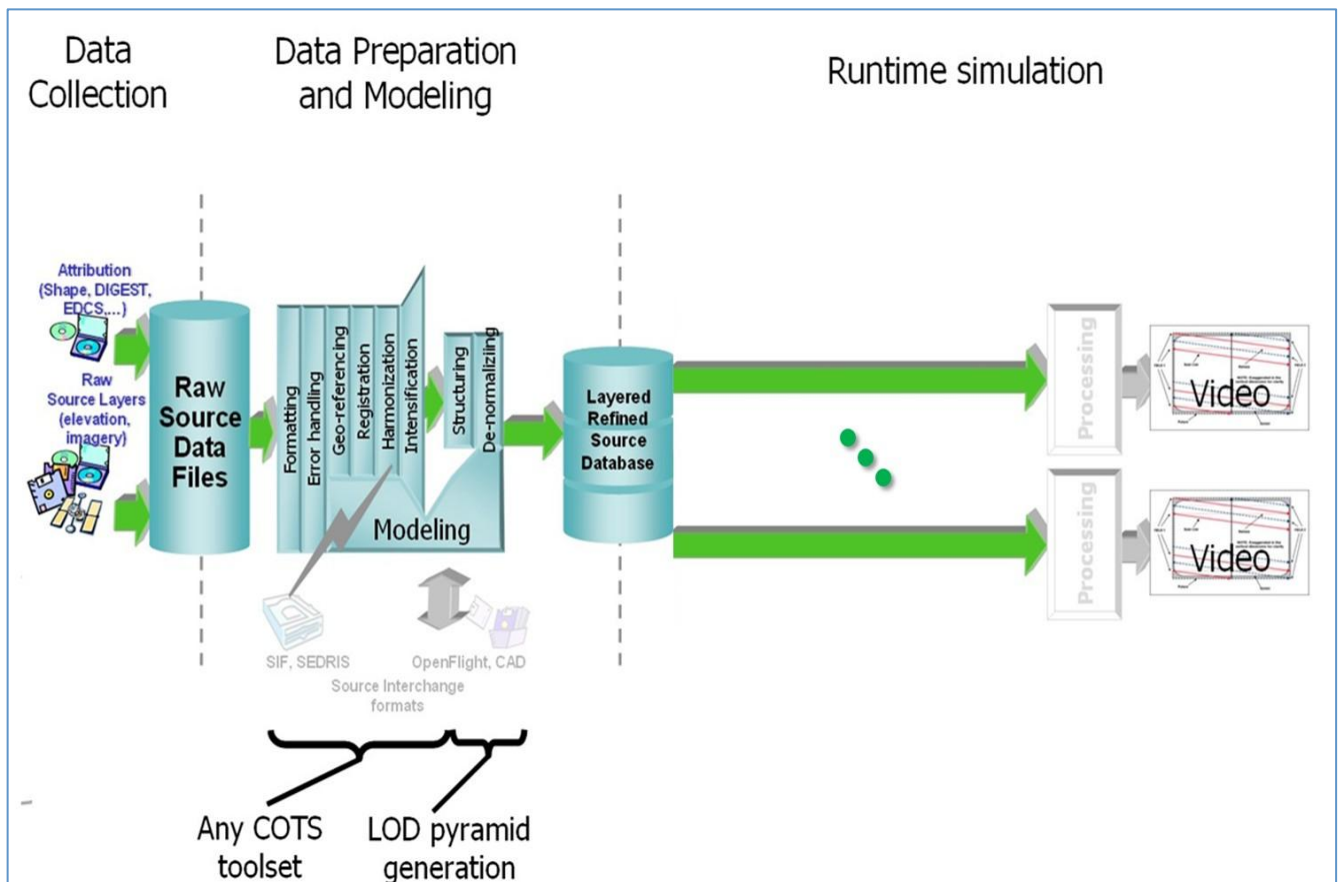
Figure 1- 4: SE Workflow with CDB as Combined Off-line/Runtime Data Store Repository
