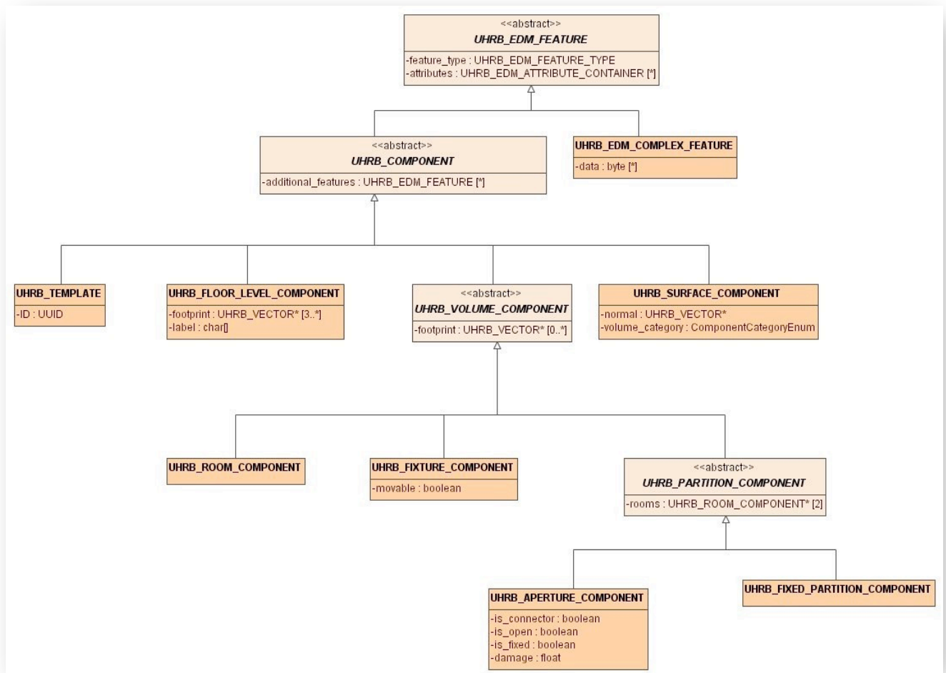
Figure 6-4: UHRB Class Diagram
