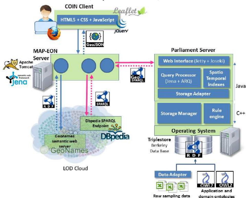
Figure 10: Architecture of COIN
