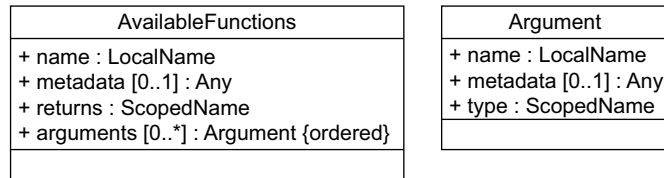
Figure 16 — AvailableFunction
