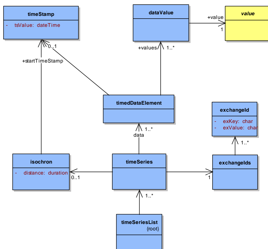
Figure 7 - The XHydro time series model
