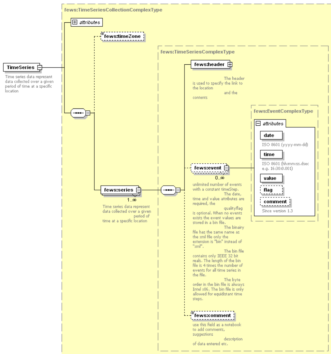
Figure 9 The DelftFEWS Published Interface time series
