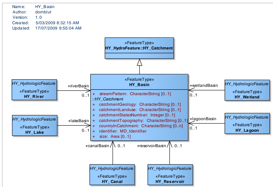
Figure 10 – Basins UML in the GRDC profile
