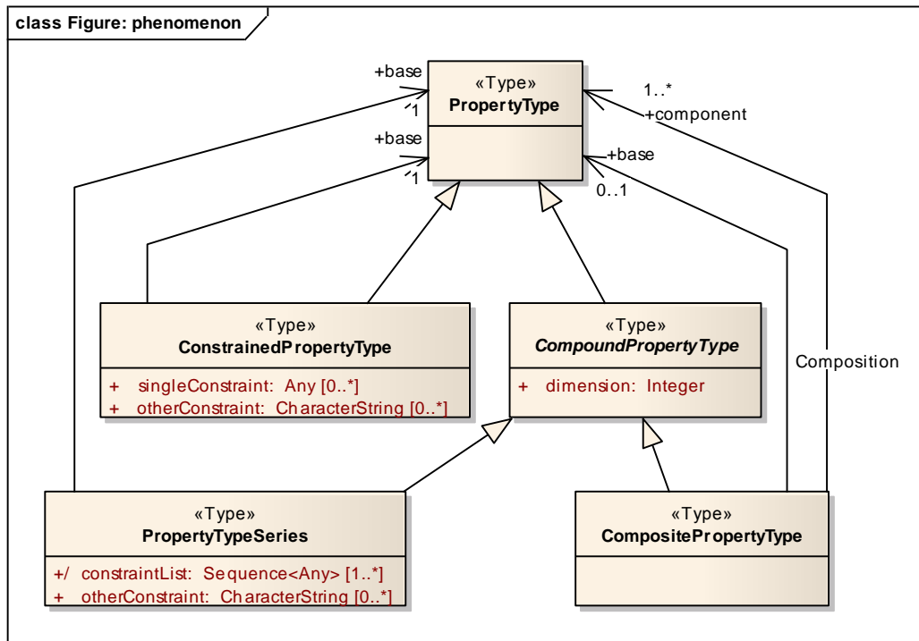
Figure 12 - SWE common phenomenon definition UML
