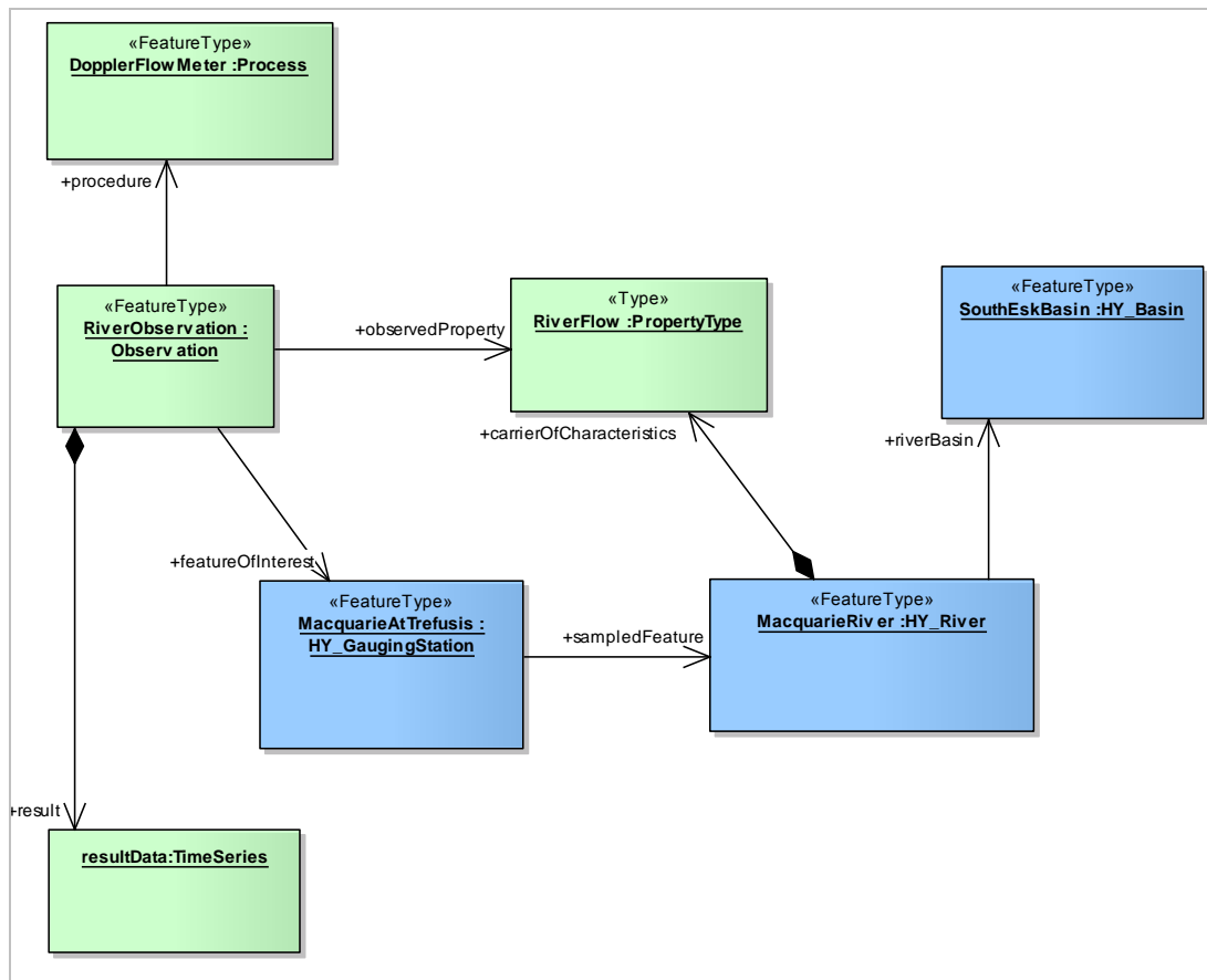
Figure 11 - Example river flow observation in UML
