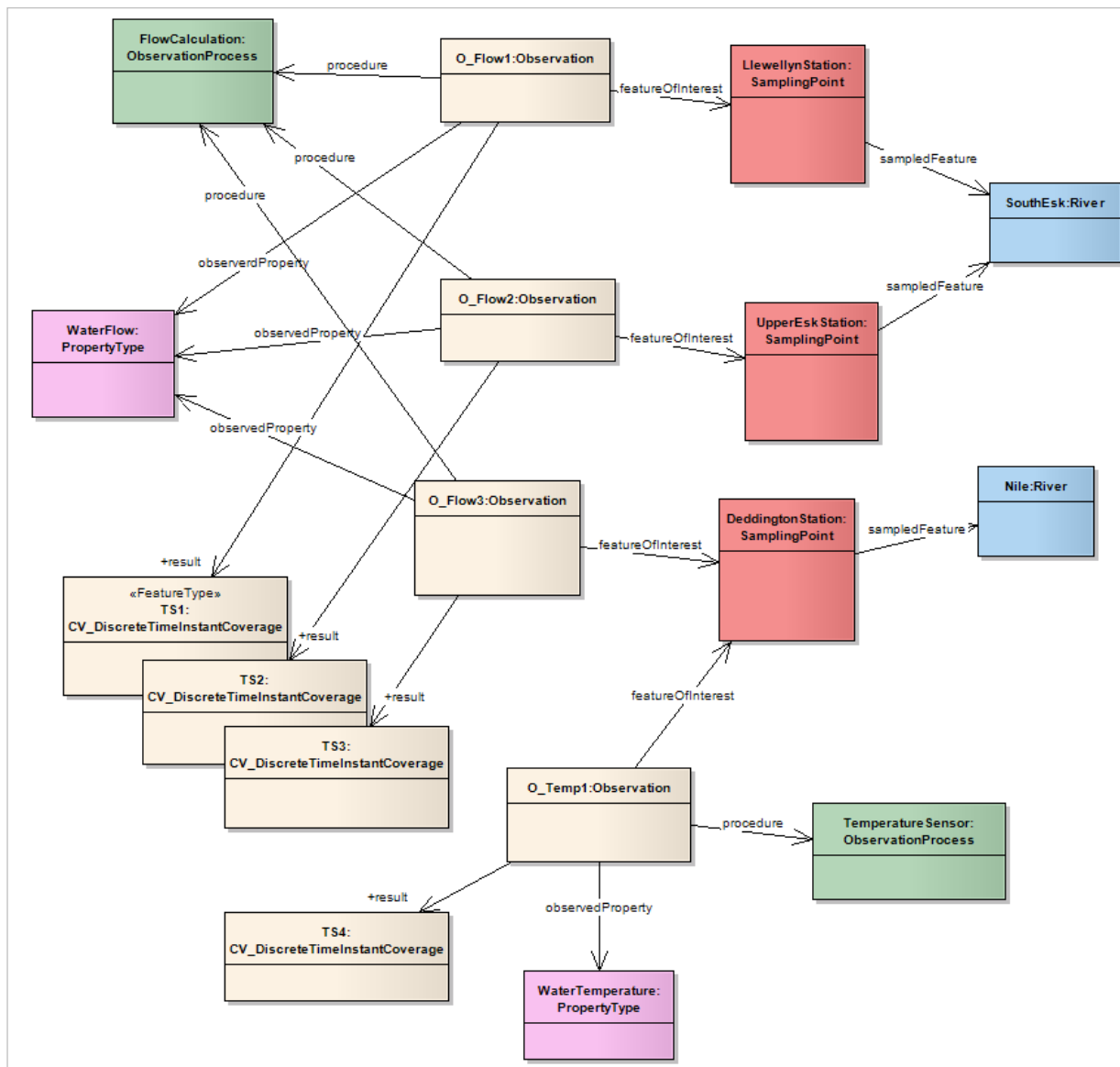
Figure 4 - Example sampling feature relationship
