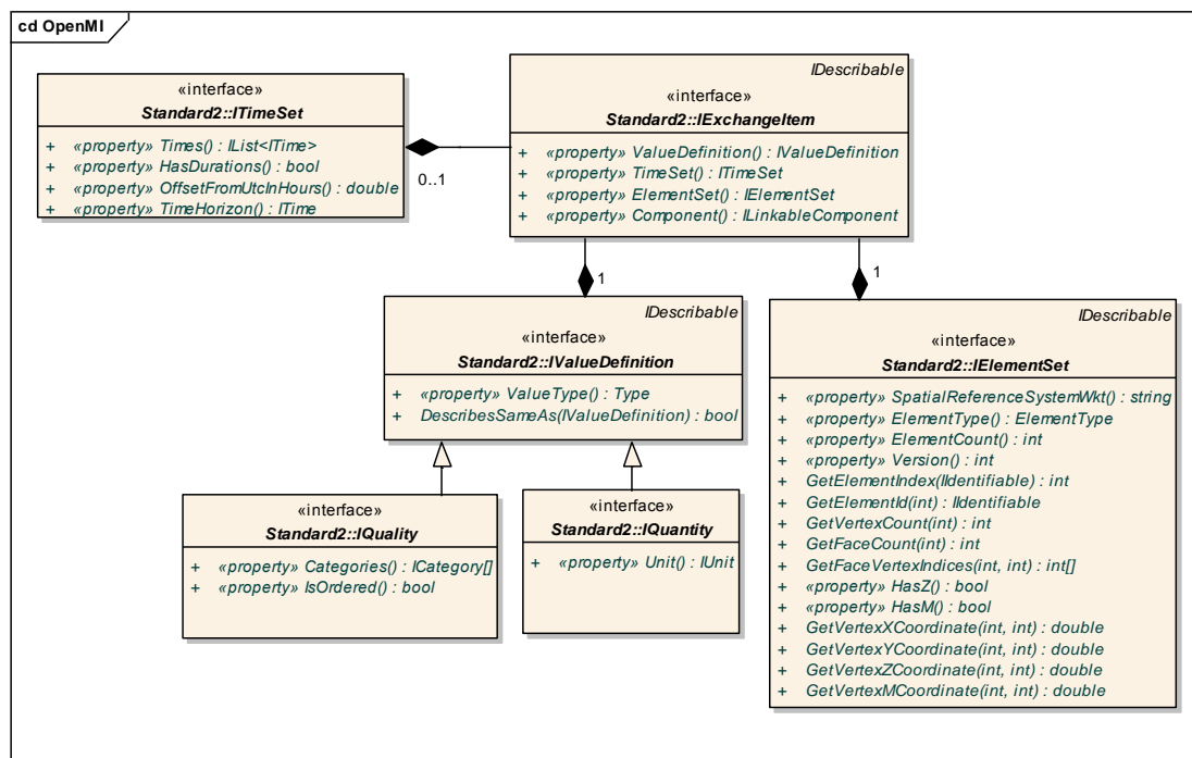
Figure 8 The OpenMI data model
