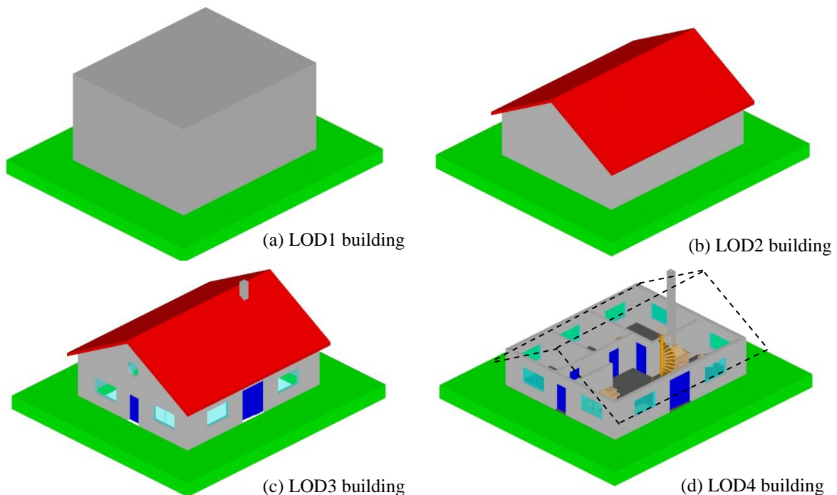
Fig. 27: Building model in LOD1 – LOD4 (source: Research Center Karlsruhe).
