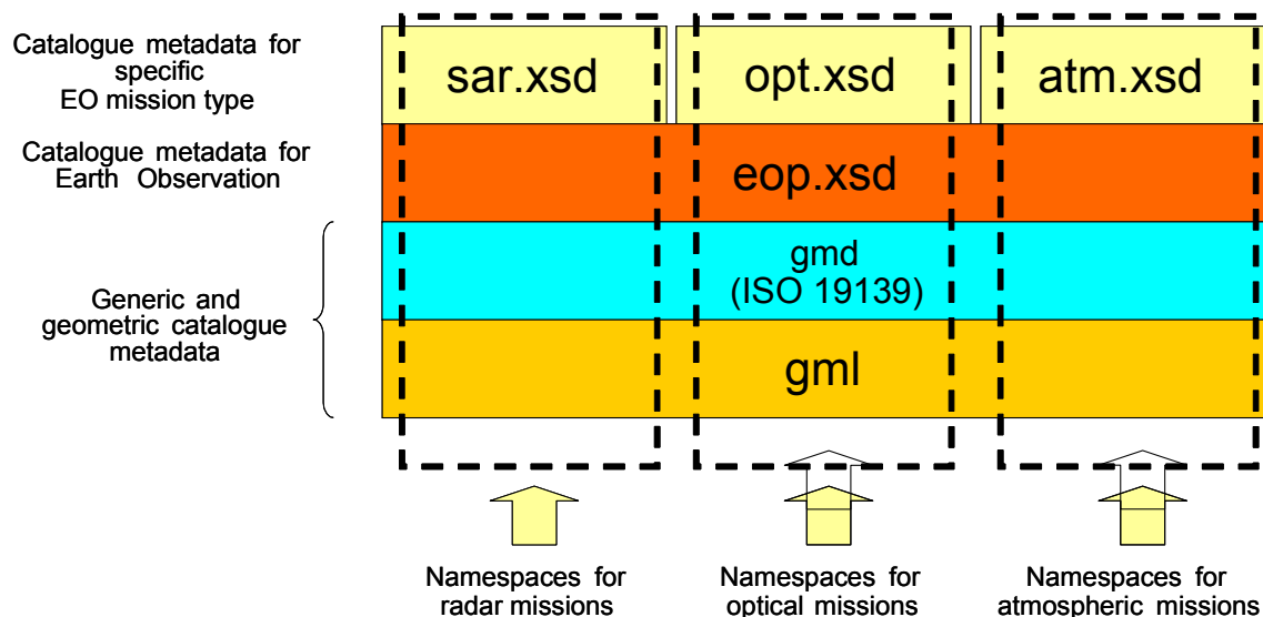
Figure 6: EO Product XML Schemas Structure
