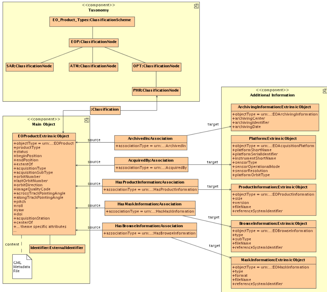
Figure 15: Complete EO Products Data Model
