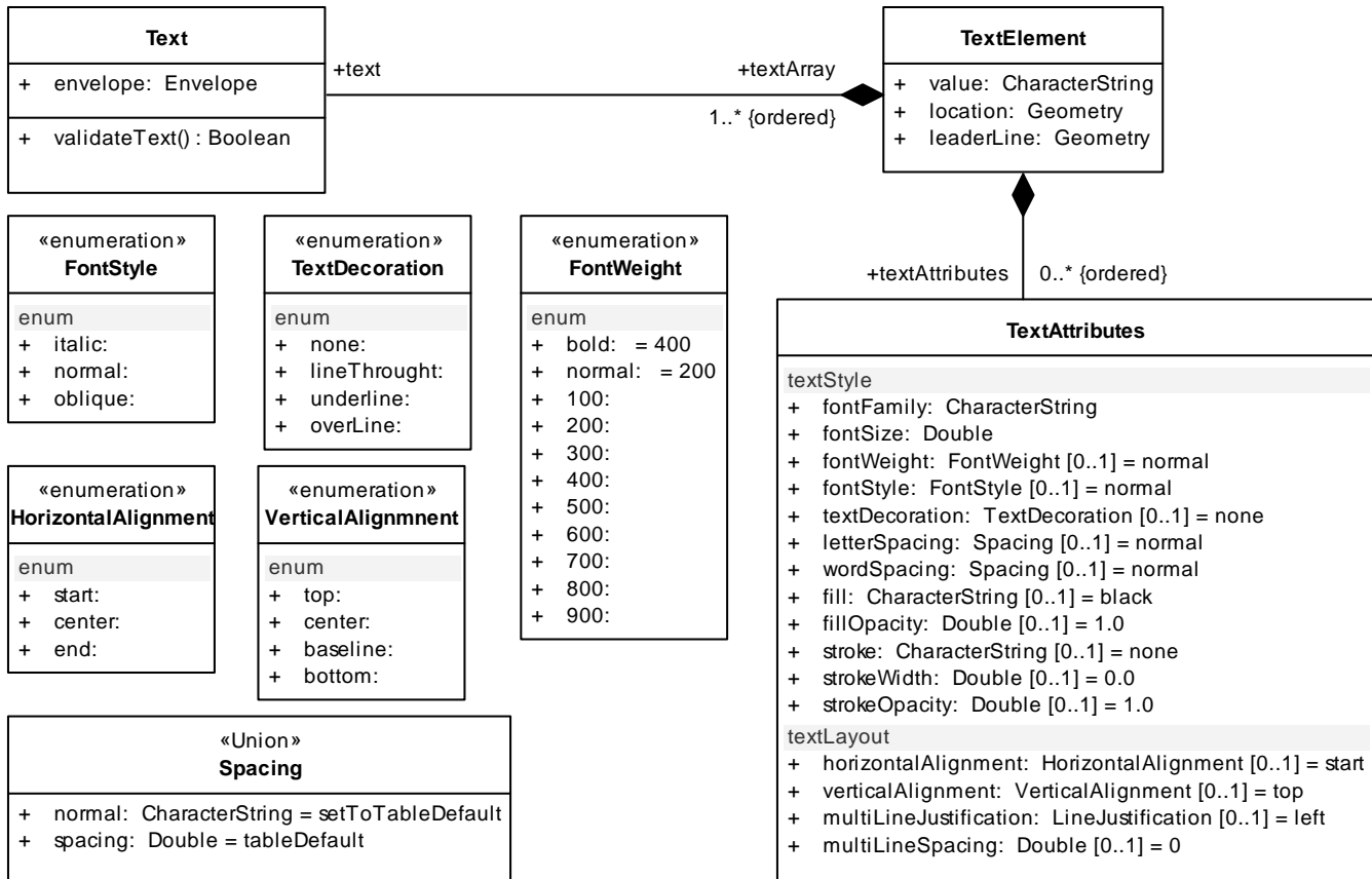
Figure 24: Text classes
