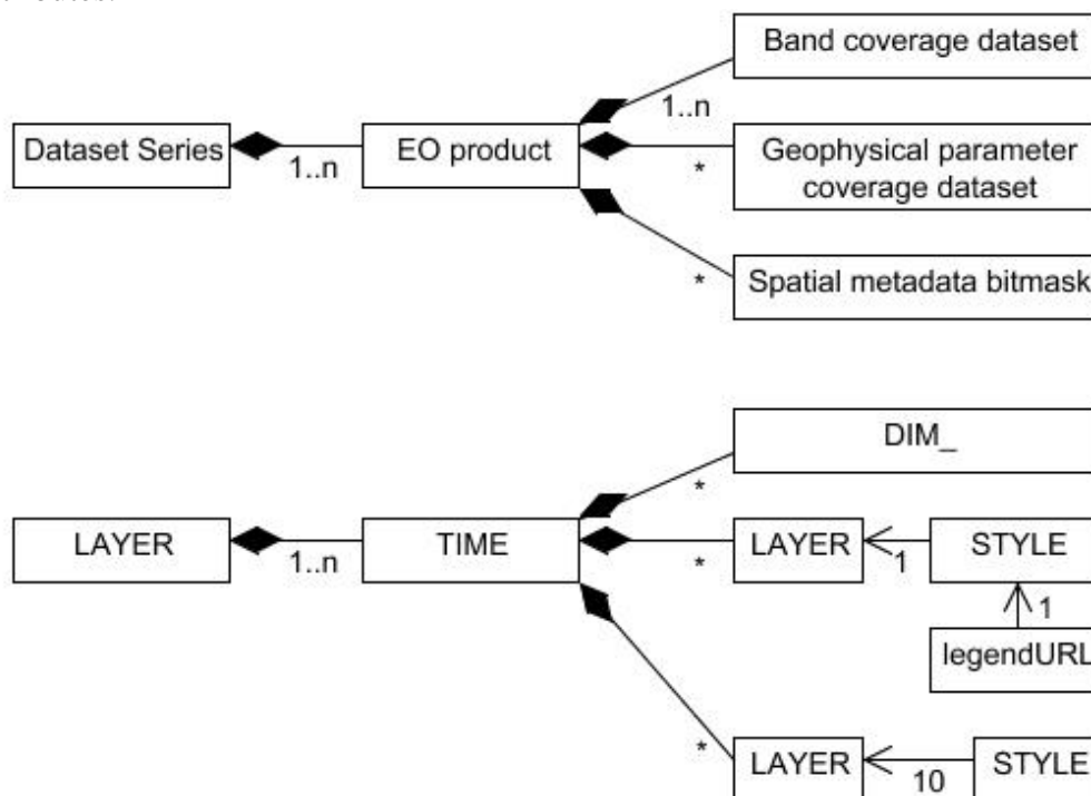
Figure 7-1: UML class diagrams showing how the organisation of EO spatial information maps to the proposed WMS service metadata model. Note the use of multiplicity on the class associations.
