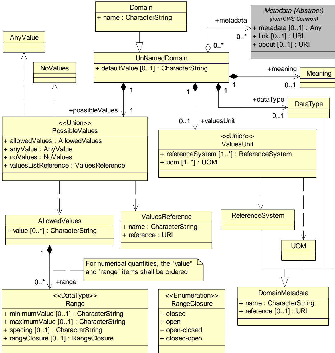
Figure E.1 — Domain package class diagram
