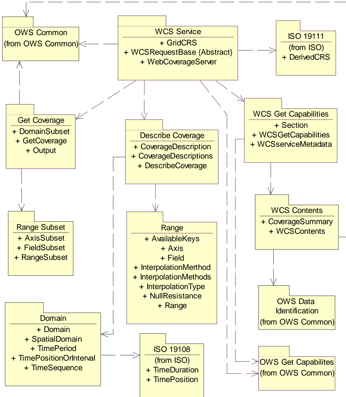
Figure D.2 — WCS interface package diagram
