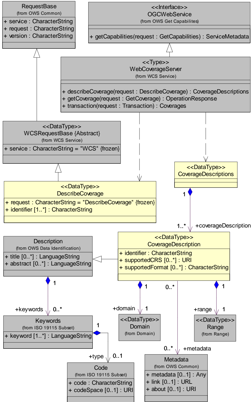
Figure D.6 — Describe Coverage package class diagram
