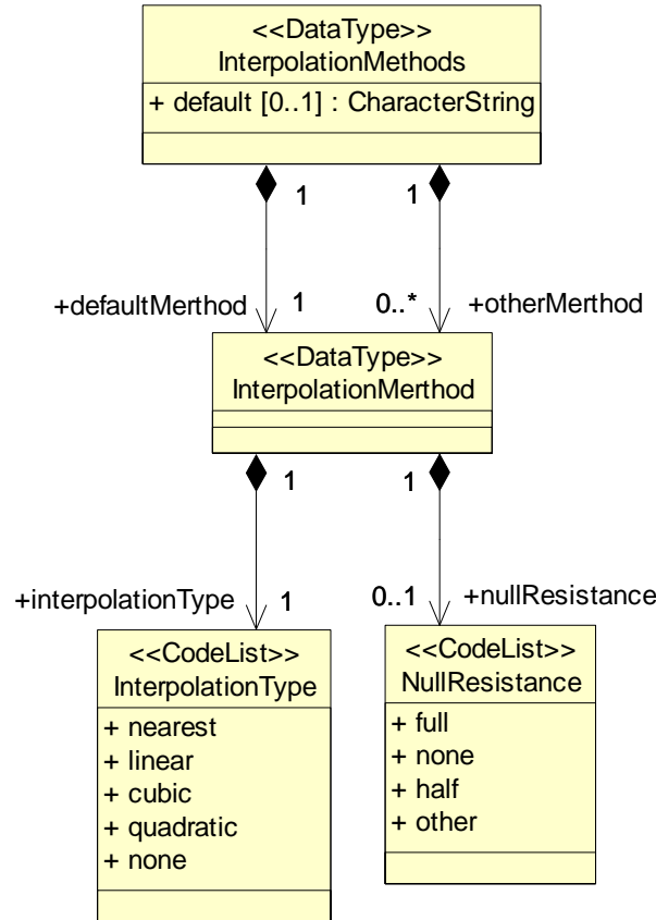
Figure I.3 — Interpolation Methods class diagram
