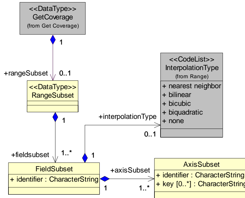
Figure D.5 — Range Subset package class diagram
