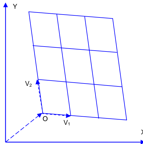
Figure H.1 — Parallelogram grid within a 2D X-Y space
