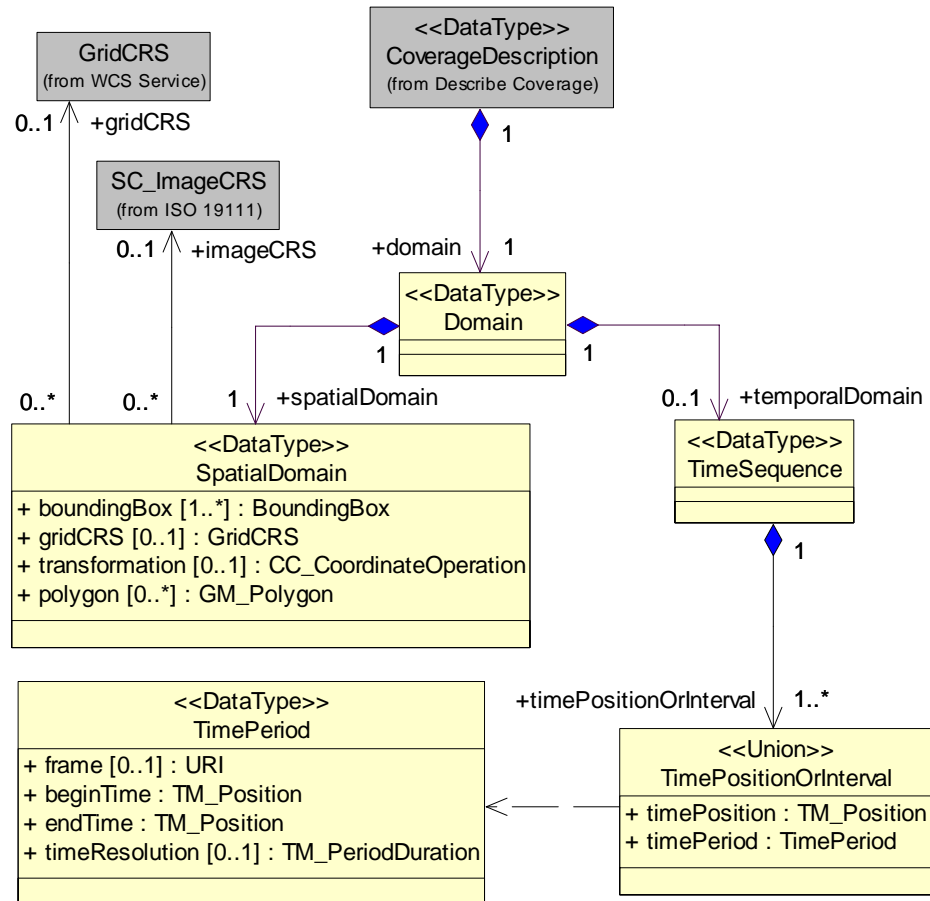
Figure D.7 — Domain package class diagram
