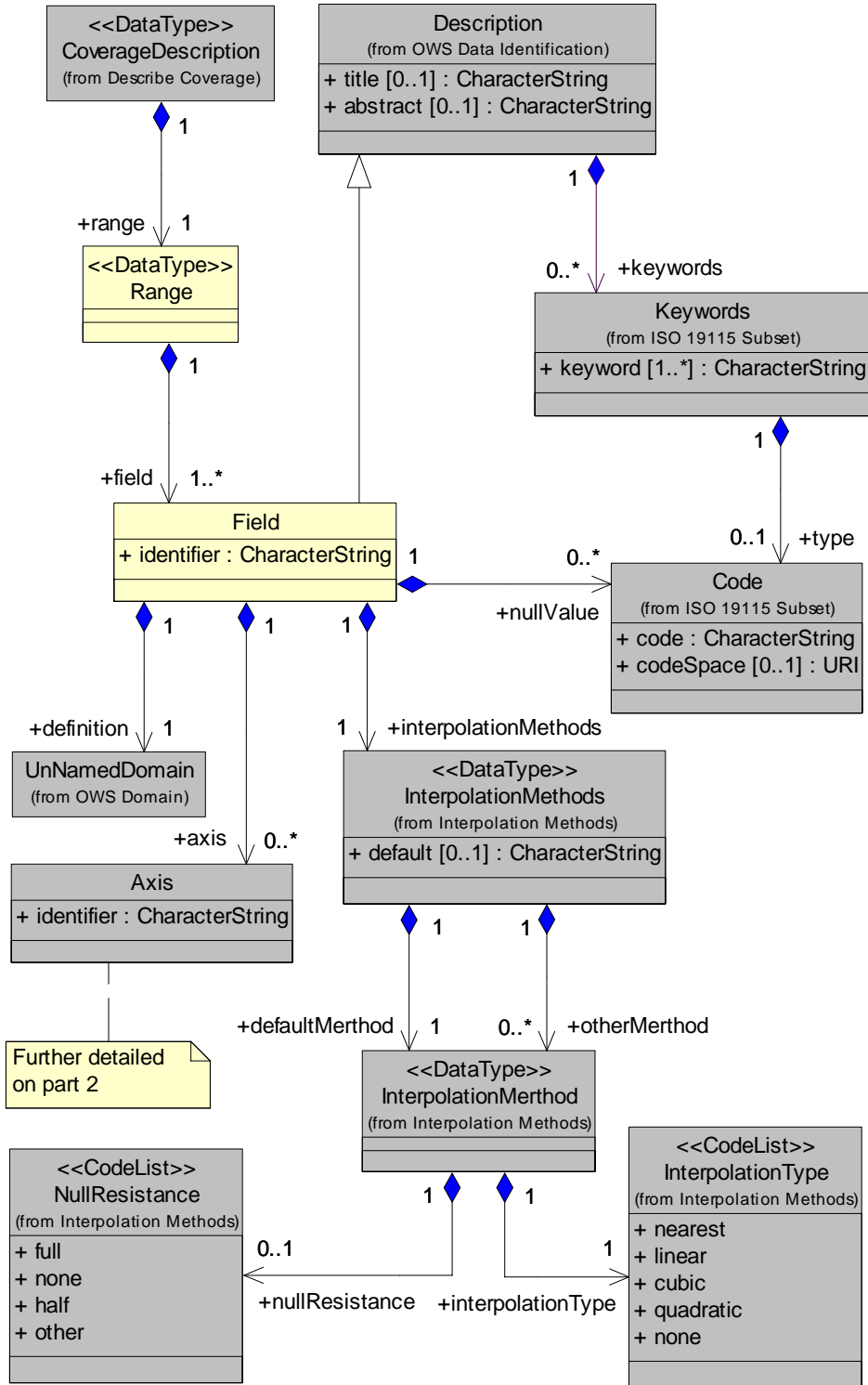
Figure 8 — Range UML class diagram, part 1
