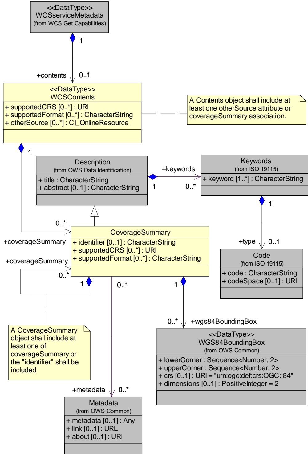
Figure 4 — Contents UML class diagram
