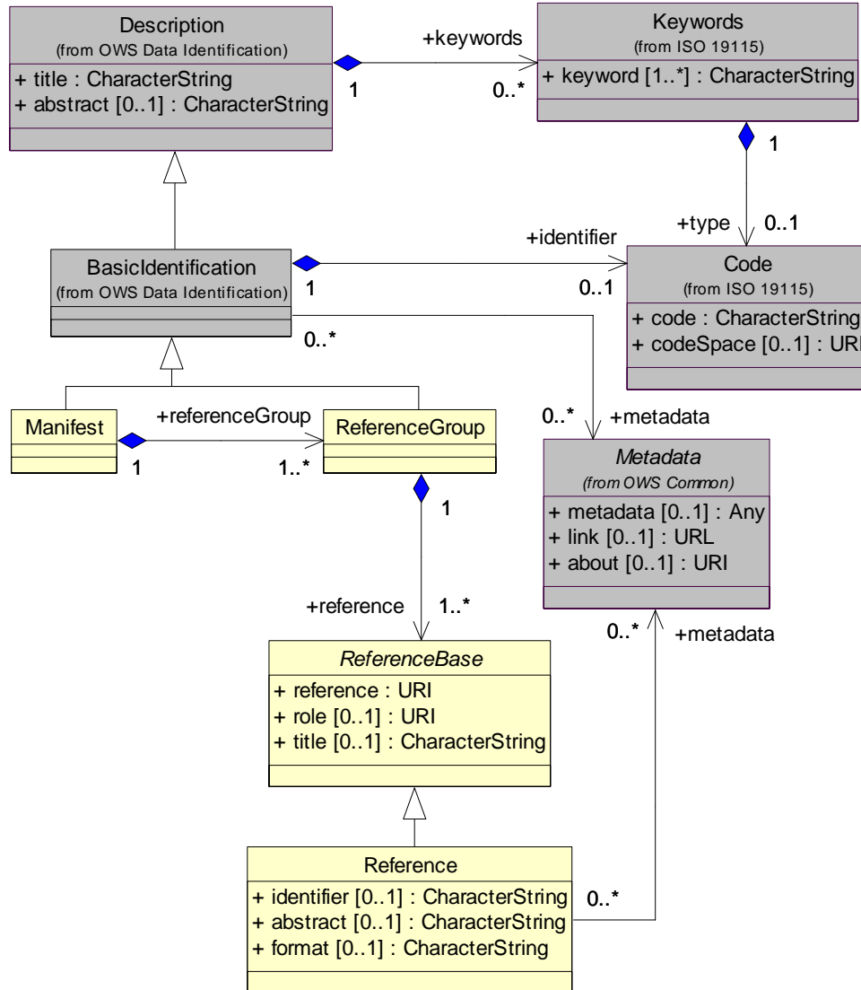
Figure I.1 — Manifest UML package
