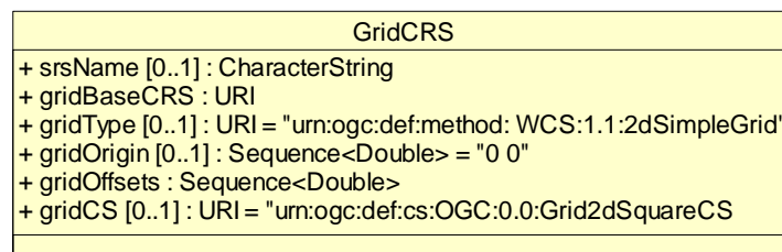
Figure G.1 — GridCRS class diagram
