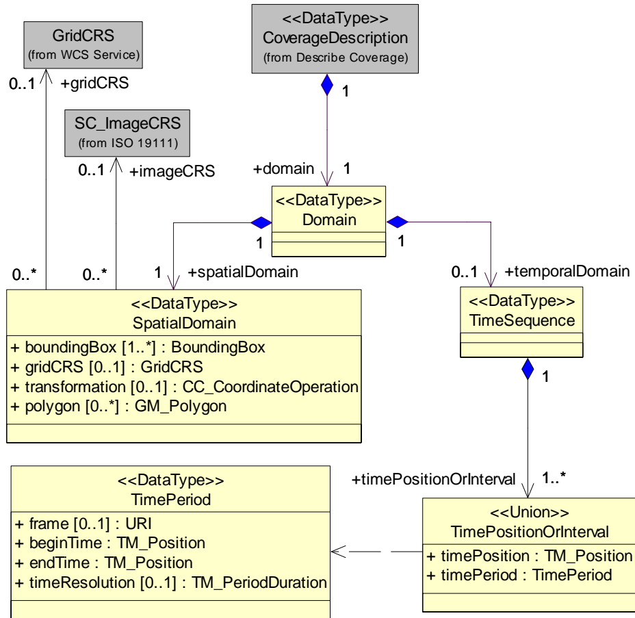
Figure 7 — Domain UML class diagram
