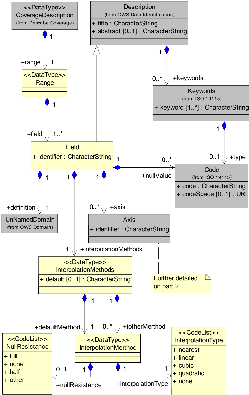
Figure D.8 — Range package class diagram, part 1
