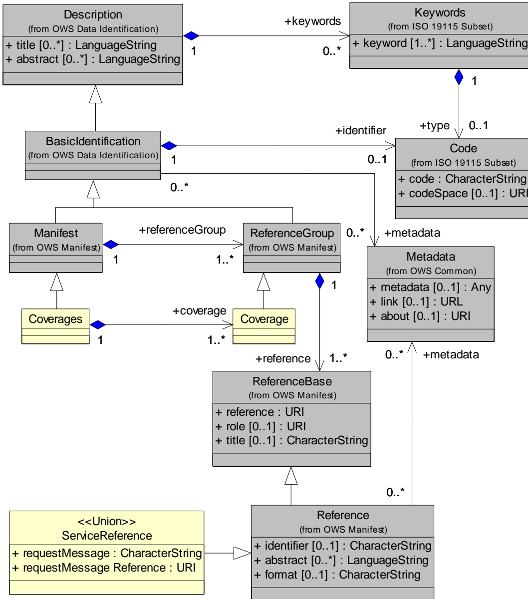
Figure I.2 — Coverage Group package partial UML diagram
