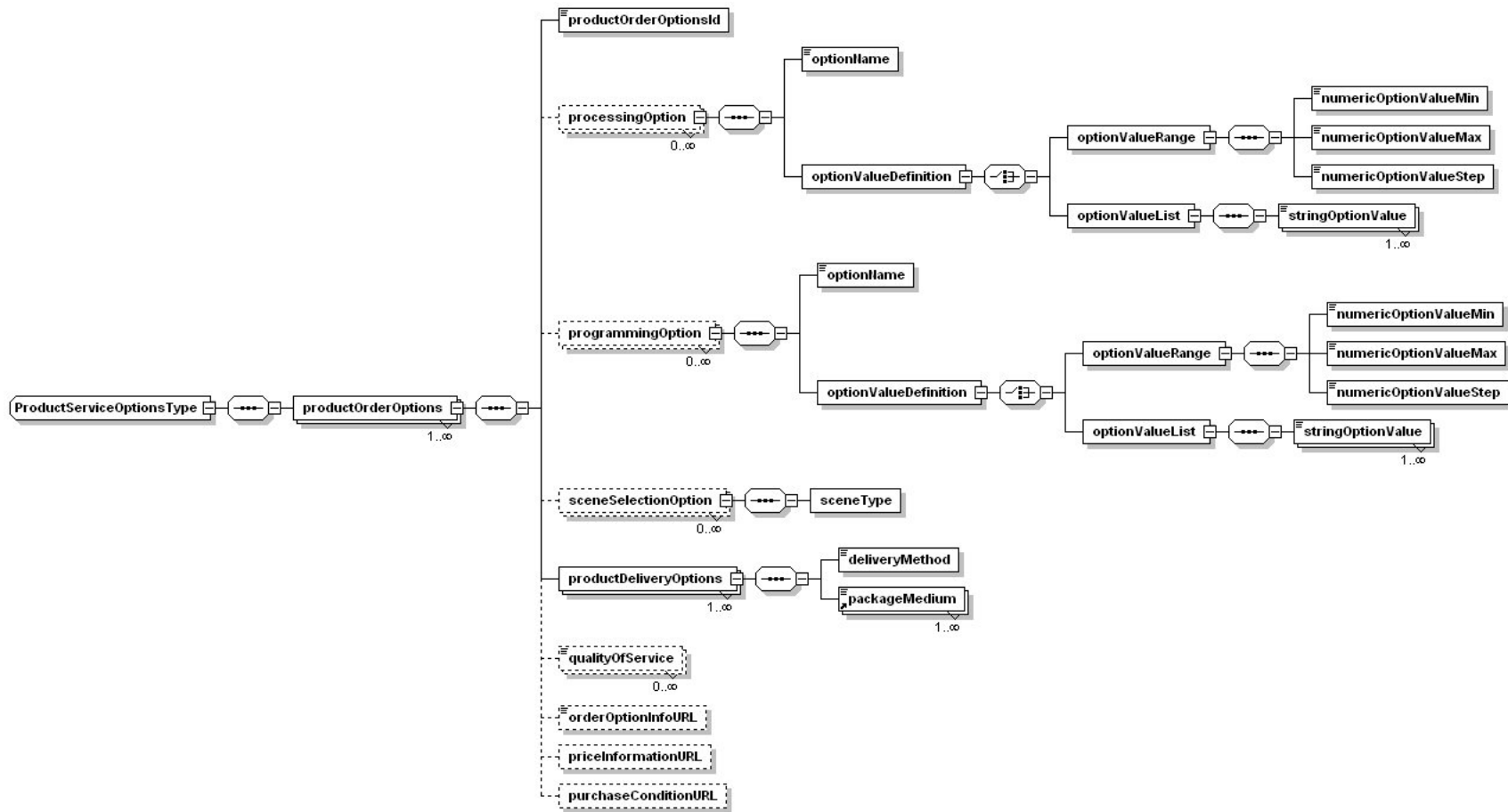
Figure 8-1: ProductServiceOptions Type Diagram.
