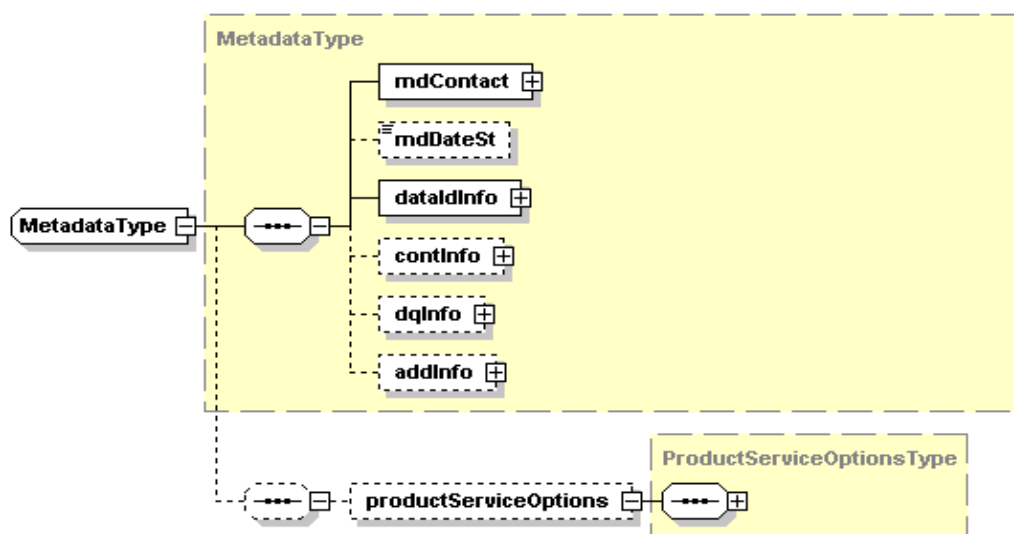
Figure 8-4: Metadata Type Diagram
