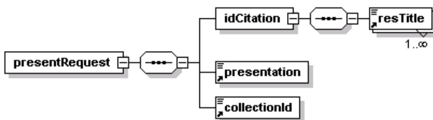
Figure 7-3: PresentRequest Diagram
