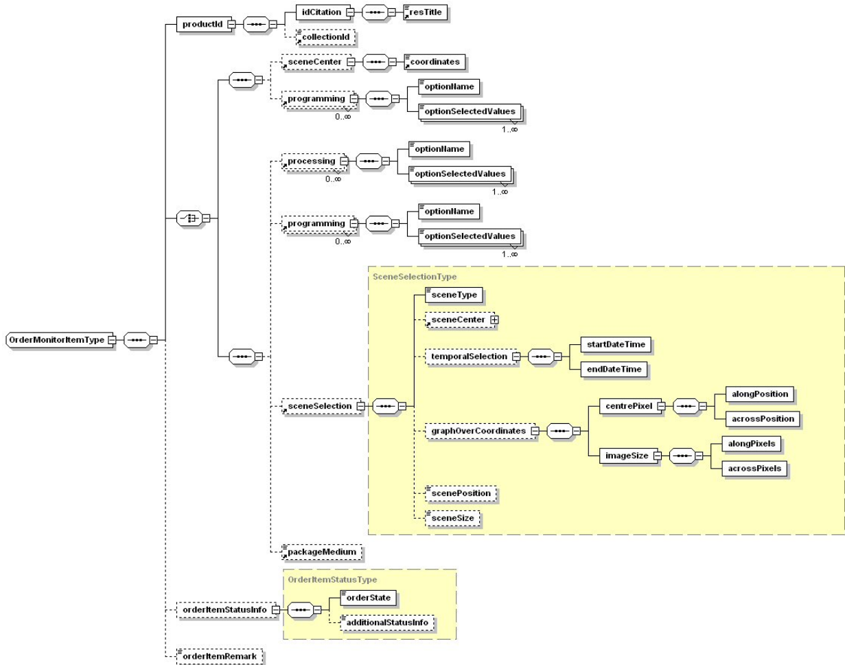
Figure 8-12: OrderMonitorItem diagram.
