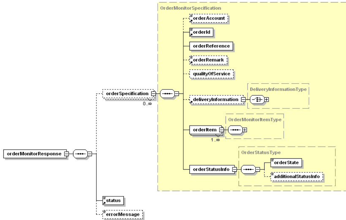
Figure 8-11: OrderMonitorResponse element.
