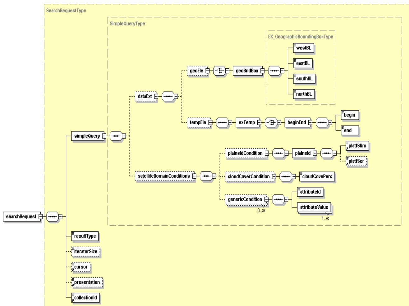
Figure 7-2: SearchRequest Diagram.
