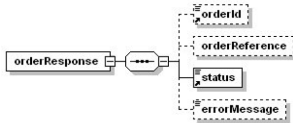
Figure 8-9: OrderResponse element diagram.
