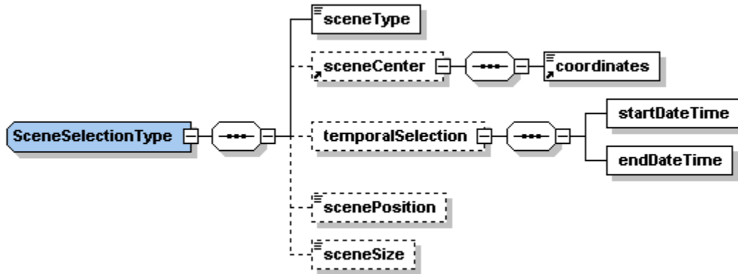
Figure 8-8: SceneSelectionOptions Type diagram
