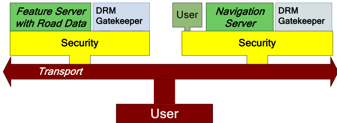
Figure 3: Topology for complex gatekeeper example
