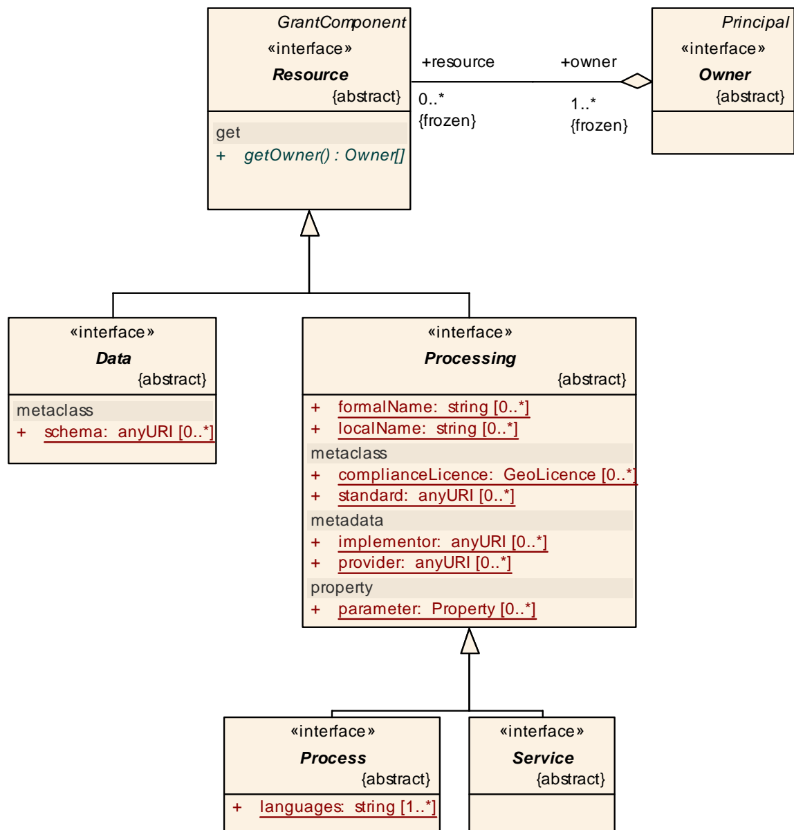
Figure B – 10: Resources
