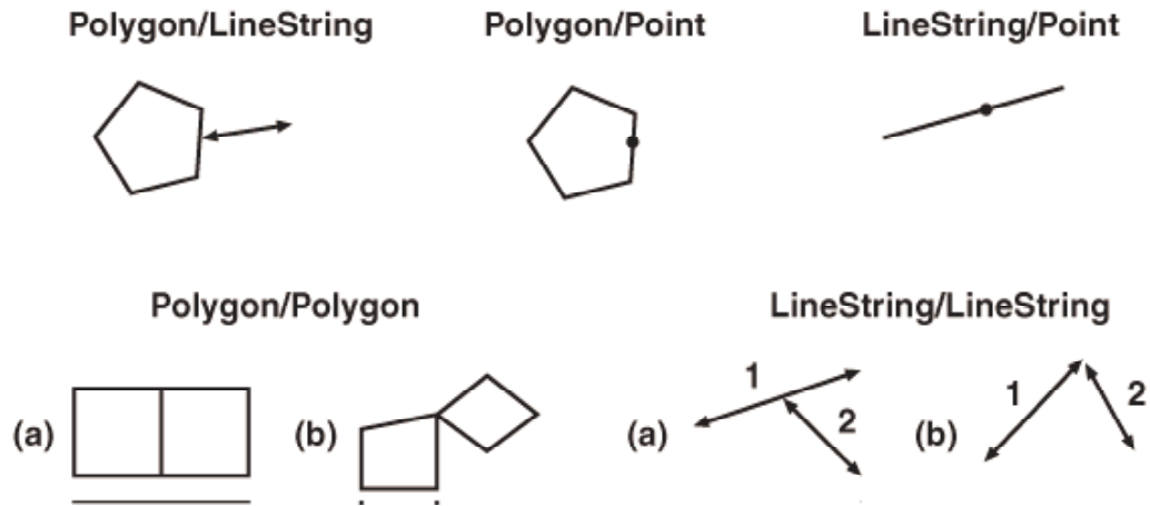
Figure 9 — Examples of the Touches relationship
