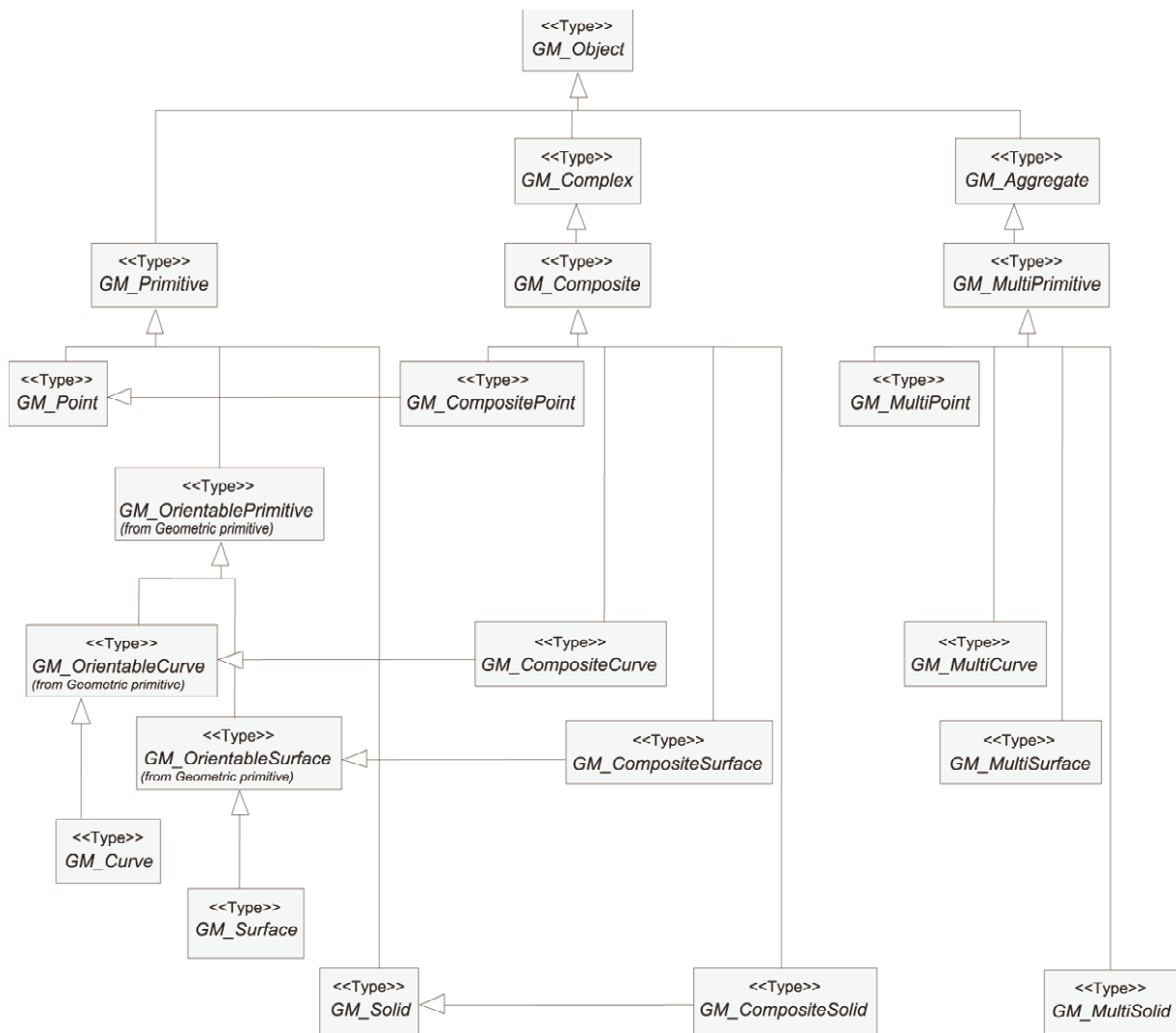
Figure A.1 — The root type and subordinates of the Spatial schema
