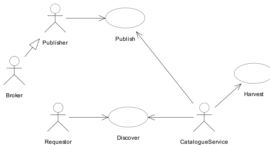
Figure 2: Overall system use cases
