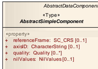
Figure 7.7 – AbstractSimpleComponent Class
