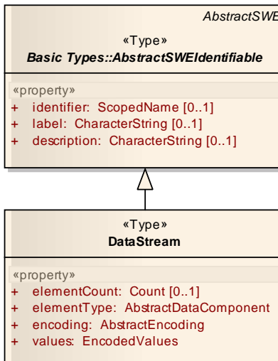
Figure 7.31 – DataStream Class
