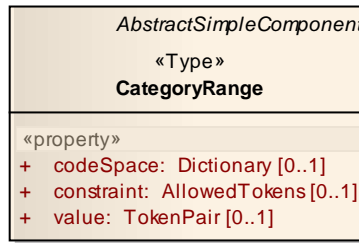
Figure 7.14 – CategoryRange Class
