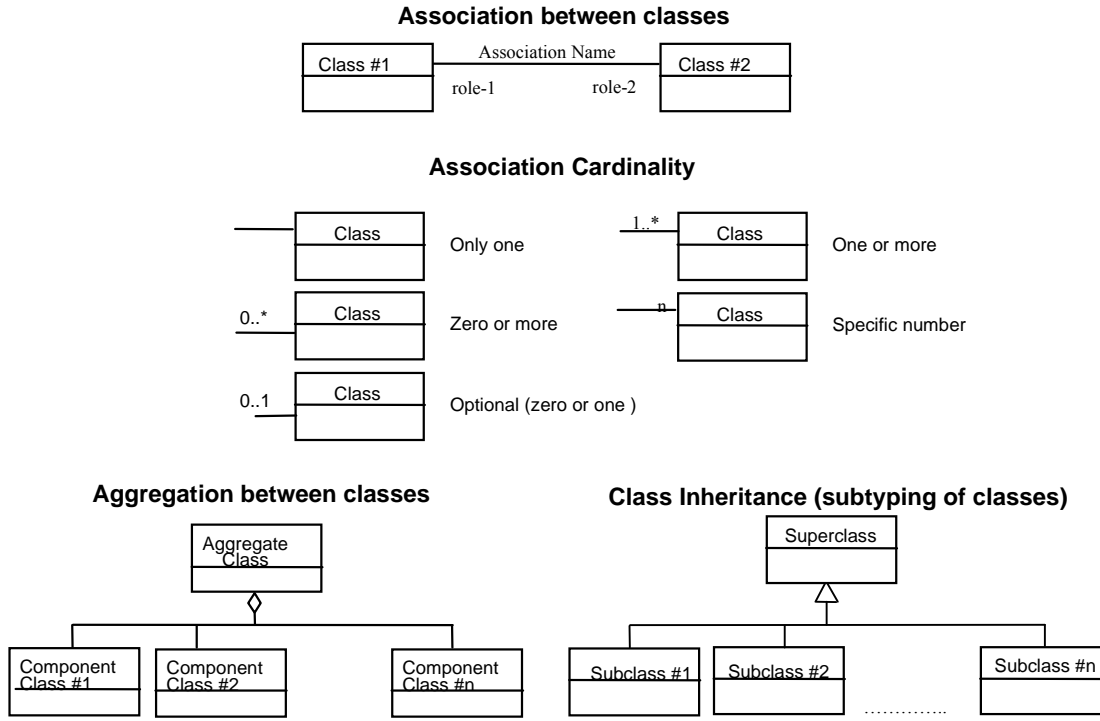
Figure 5.1 – UML Notation
