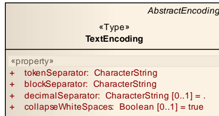
Figure 7.33 – TextEncoding Class
