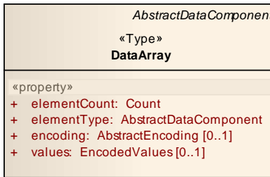
Figure 7.29 – DataArray Class
