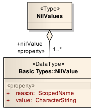
Figure 7.19 – NilValues Class
