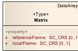
Figure 7.30 – Matrix Class
