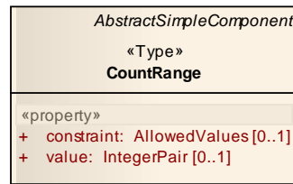
Figure 7.15 – CountRange Class
