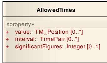
Figure 7.22 – AllowedTimes Class
