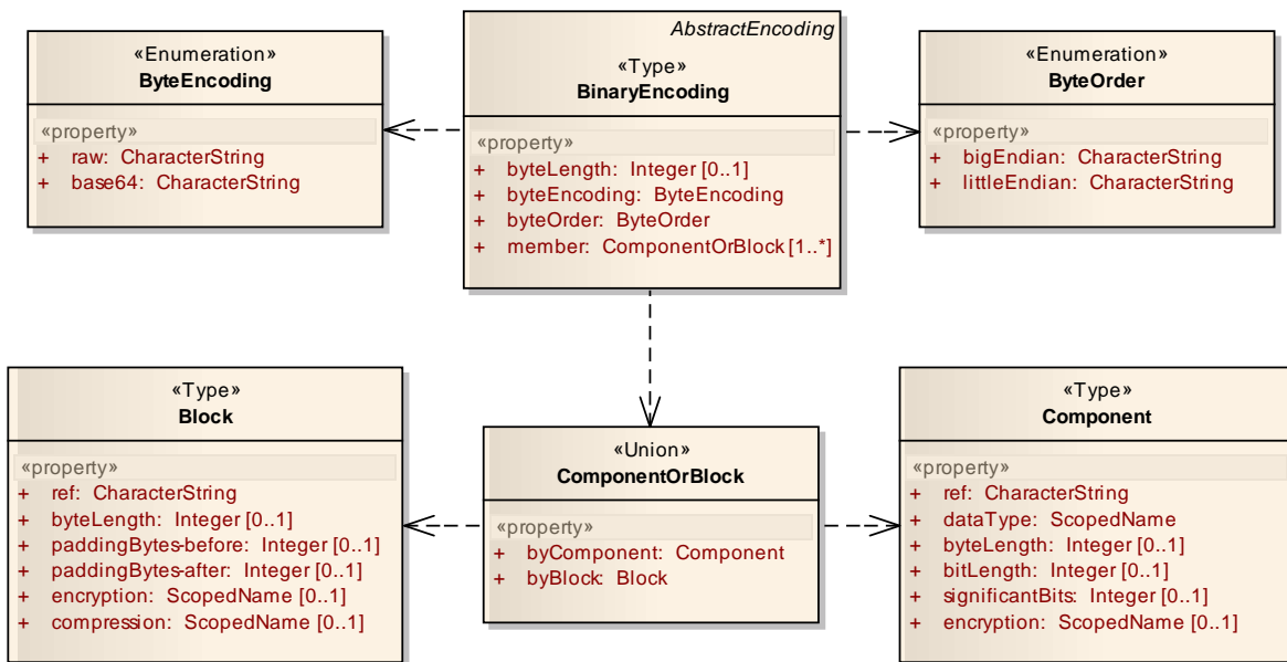
Figure 7.35 – BinaryEncoding Class
