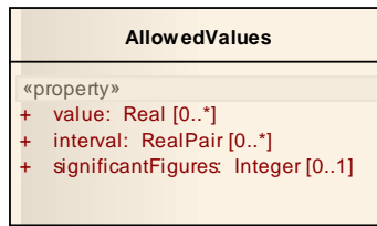
Figure 7.21 – AllowedValues Class
