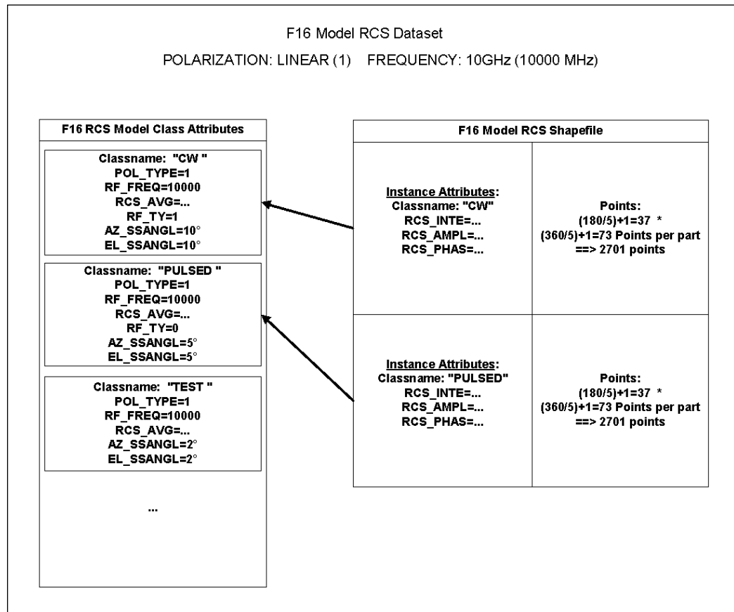
Figure 7-5: Example of RCS Vector Data
