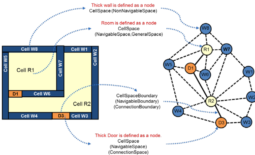
b) Example for Thick Door Model
