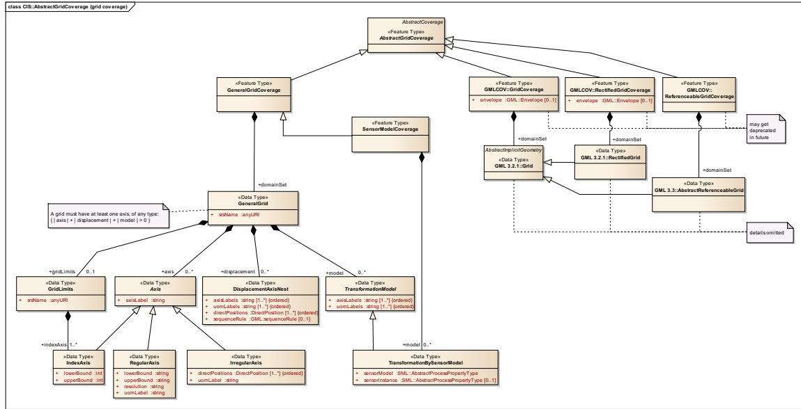
Figure 16: Grid coverages
