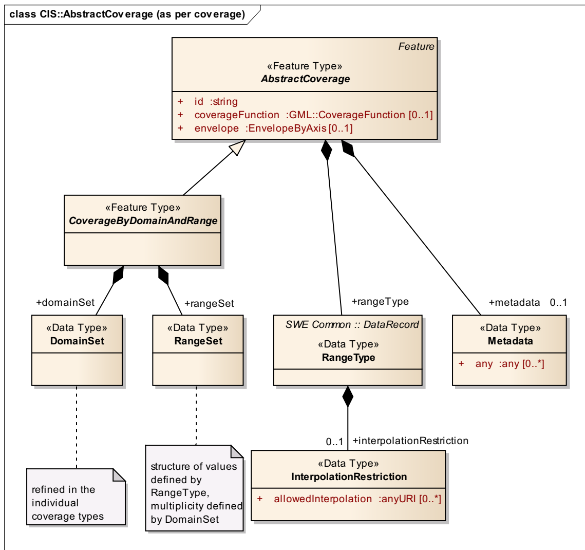
Figure 2: CIS : : AbstractCoverage structure (as per class coverage)
