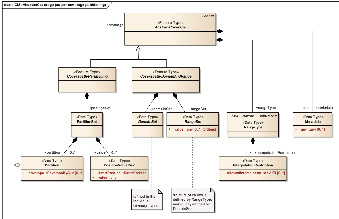
Figure 12: UML diagram of CIS::CoverageByPartitioning structure as per coverage-partitioning
