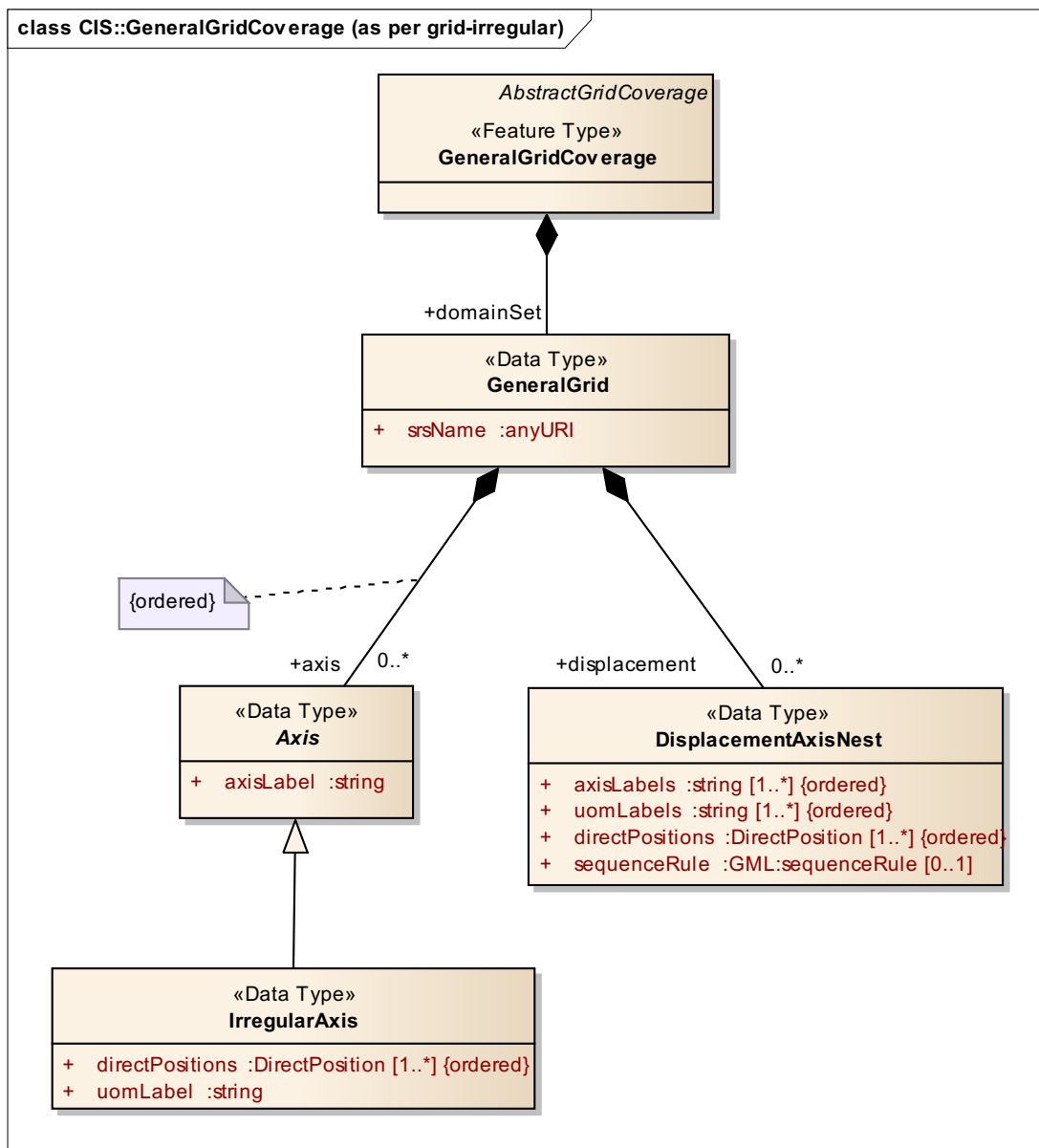
Figure 8: UML diagram of CIS::GeneralGrid structure as per grid-irregular
