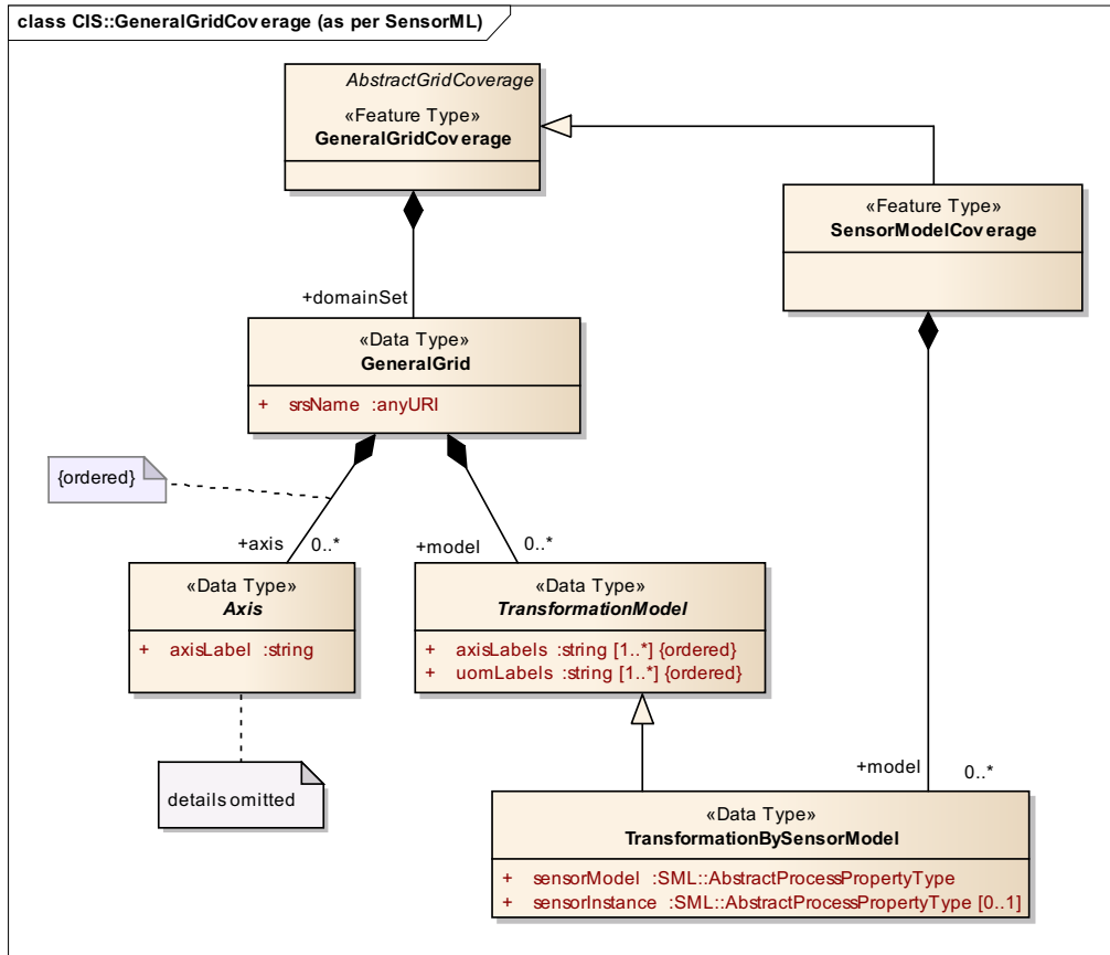
Figure 10: UML diagram of CIS::GeneralGridCoverage structure as per SensorML
