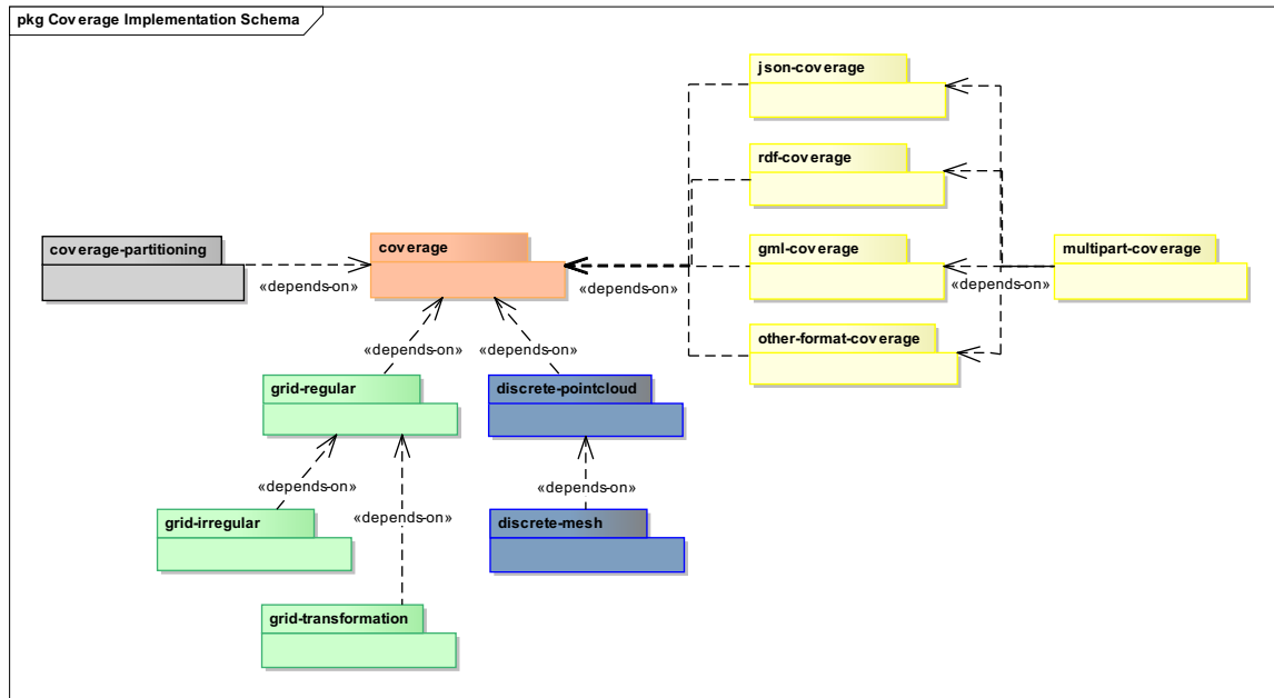
Figure 1: The Coverage class hierarchy as UML package diagram
