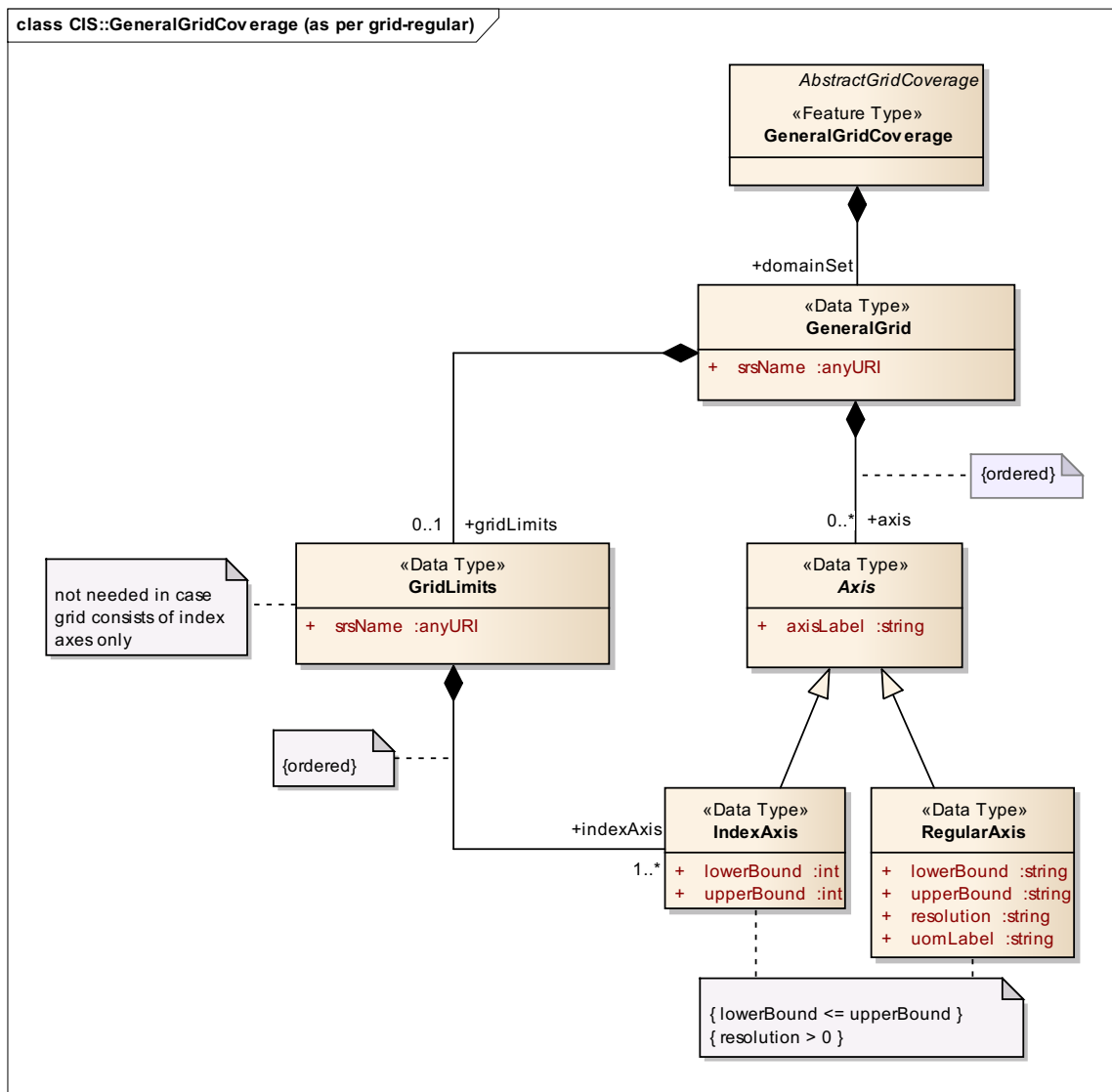
Figure 5: CIS::GeneralGridCoverage structure as per grid-regular
