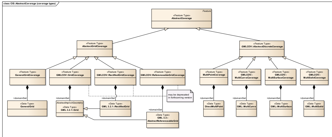
Figure 14: Coverage types
