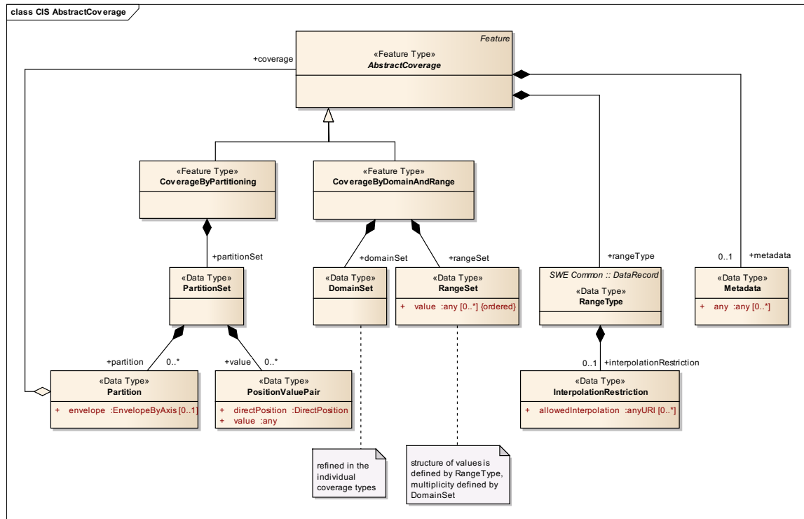
Figure 15: Coverage structure
