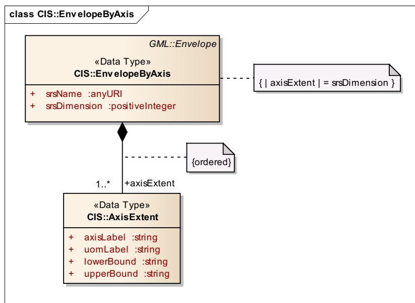
Figure 4: CIS::EnvelopeByAxis structure
