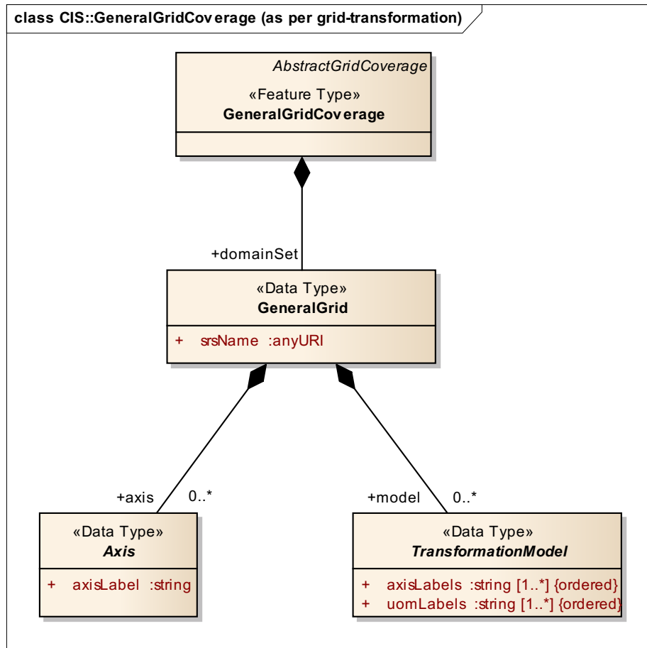
Figure 9: UML diagram of CIS::GeneralGridCoverage structure as per grid-transformation
