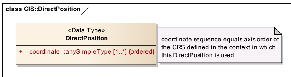
Figure 3: CIS::DirectPosition structure
