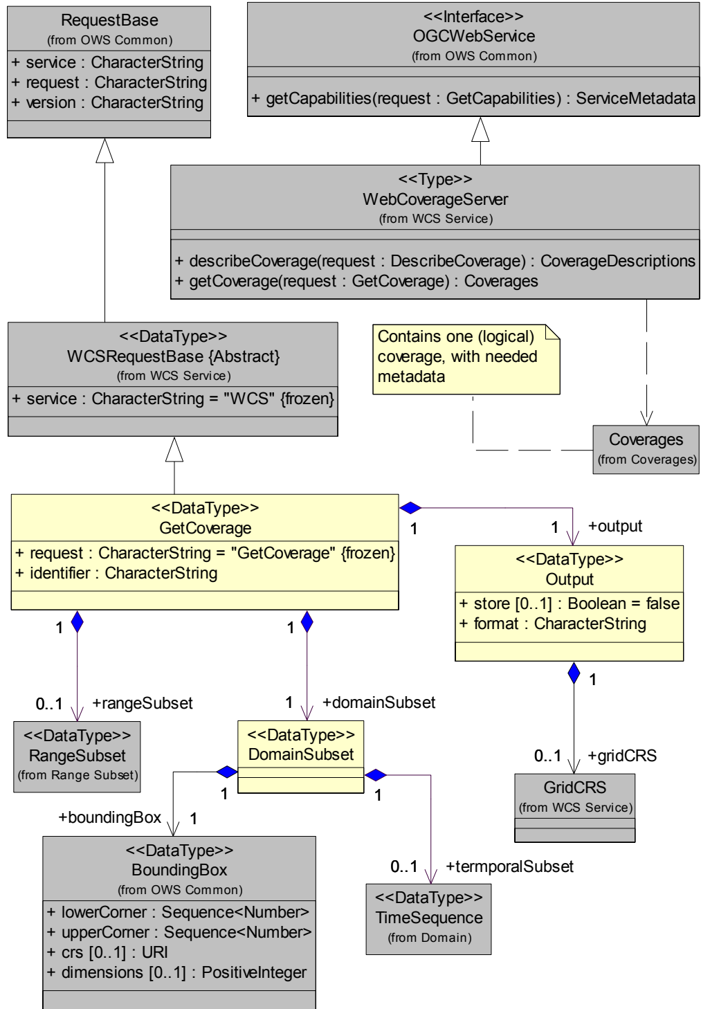
Figure D.4 — Get Coverage package class diagram
