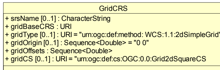
Figure F.1 — GridCRS class diagram
