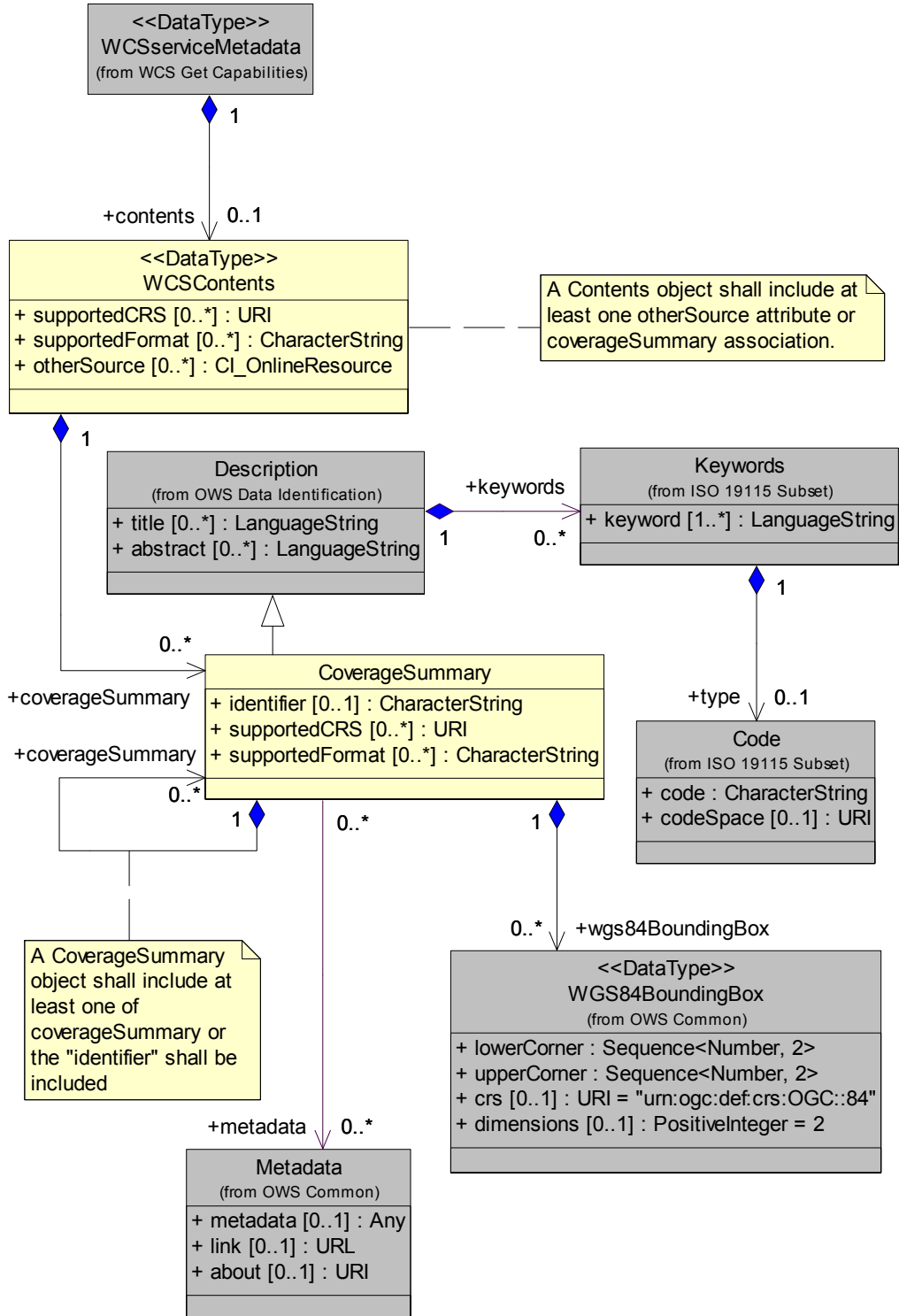
Figure D.11 — WCS Contents package class diagram
