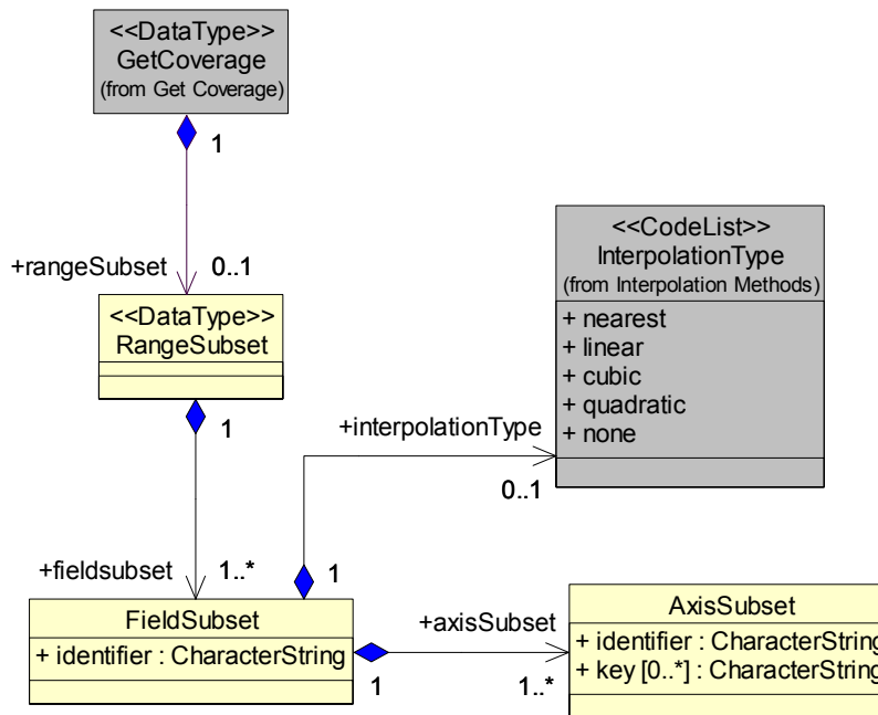
Figure D.5 — Range Subset package class diagram
