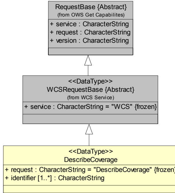
Figure 5 — DescribeCoverage operation request UML class diagram
